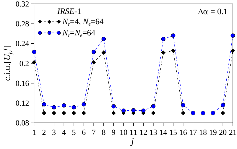
Figure 13. Coefficient of interval uncertainty of the selected nodal displacements in the load direction of the plate (LC2) discretized into N_e = 64 FEs provided by the IRSE-1 considering N_r = N_e = 64 and N_r = 4 regions with uncertain Young's moduli ( \Delta\alpha = 0.1 ).
