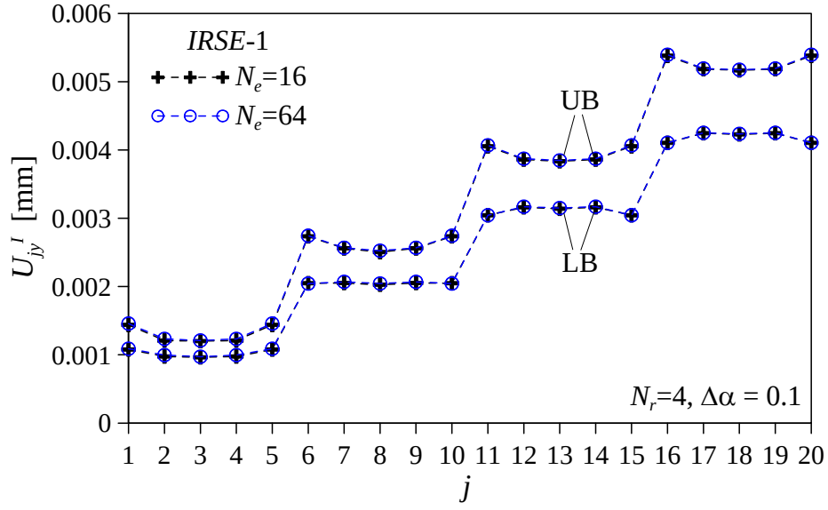
Figure 9. LB and UB of the nodal displacements in the load direction of the plate (LC1) with N_r = 4 regions with uncertain Young's moduli E^{(i)}(\alpha_i^I) = E_0^{(i)}(1 + \Delta\alpha \hat{e}_i^I) , i = 1, 2, 3, 4 , ( \Delta\alpha = 0.1 ): comparison between the estimates provided by the IRSE-1 for two different FE meshes with N_e = 16 and N_e = 64 .
