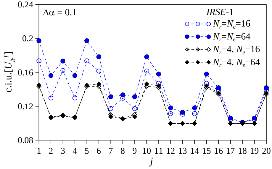
Figure 10. Coefficient of interval uncertainty of the nodal displacements in the load direction of the plate (LC1) with uncertain Young's moduli provided by the IRSE-1 for different FE ( N_e ) and uncertainty ( N_r ) meshes ( \Delta\alpha = 0.1 ).
