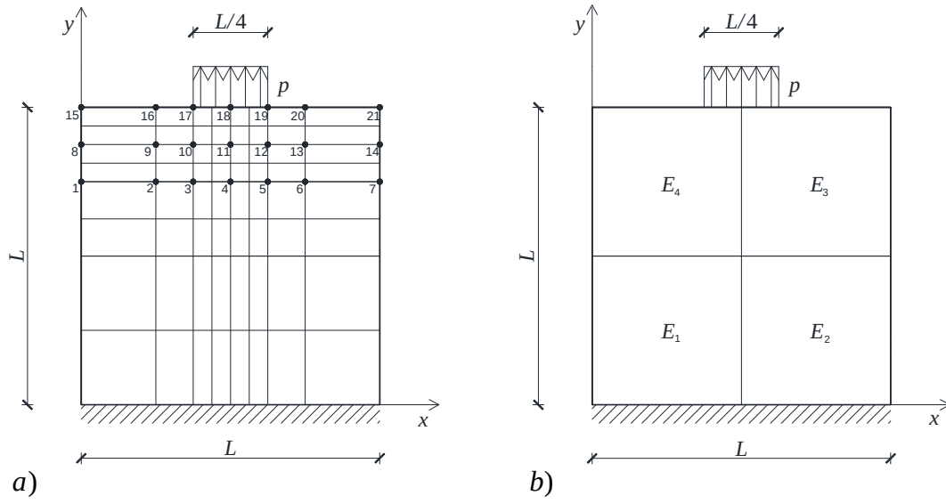
Figure 11. Square plate with uncertain Young's modulus under load condition 2 (LC2): a) FE mesh coincident with uncertainty mesh, i.e. N_e = N_r ; b) alternative uncertainty mesh consisting of N_r = 4 regions.
