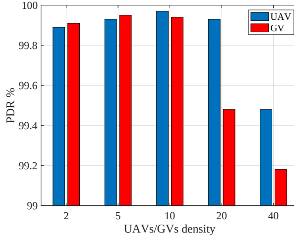
Figure 8: PDR variation vs. UAVs/GVs density.
