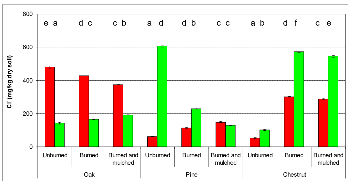
Figure 4 – Soil physico-chemical properties (mean \pm standard deviation) measured after the prescribed fire and soil mulching with fern at two survey dates (one day and one year after the fire) in the experimental forest sites (Samo, Calabria, Southern Italy).
