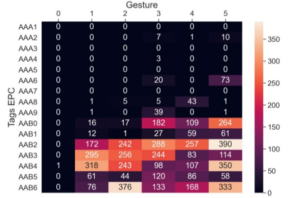
Fig. 2. Lost tags by Antenna 1 vs. gesture.
