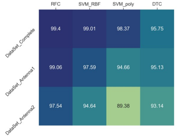
Fig. 8. Accuracy of the different models vs datasets.
