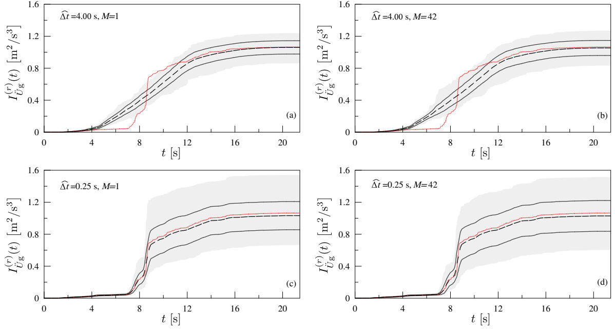
Figure 6: Cumulative intensity functions I_f(t) of the parent signal (red line) and child signals for different combinations of moving time window \widehat{\Delta t} and number M of time subdivisions (mean value, black dashed line; mean \pm one standard deviation, black solid lines; envelope of maximum and minimum values for whole set of generated signals, grey shaded area)
