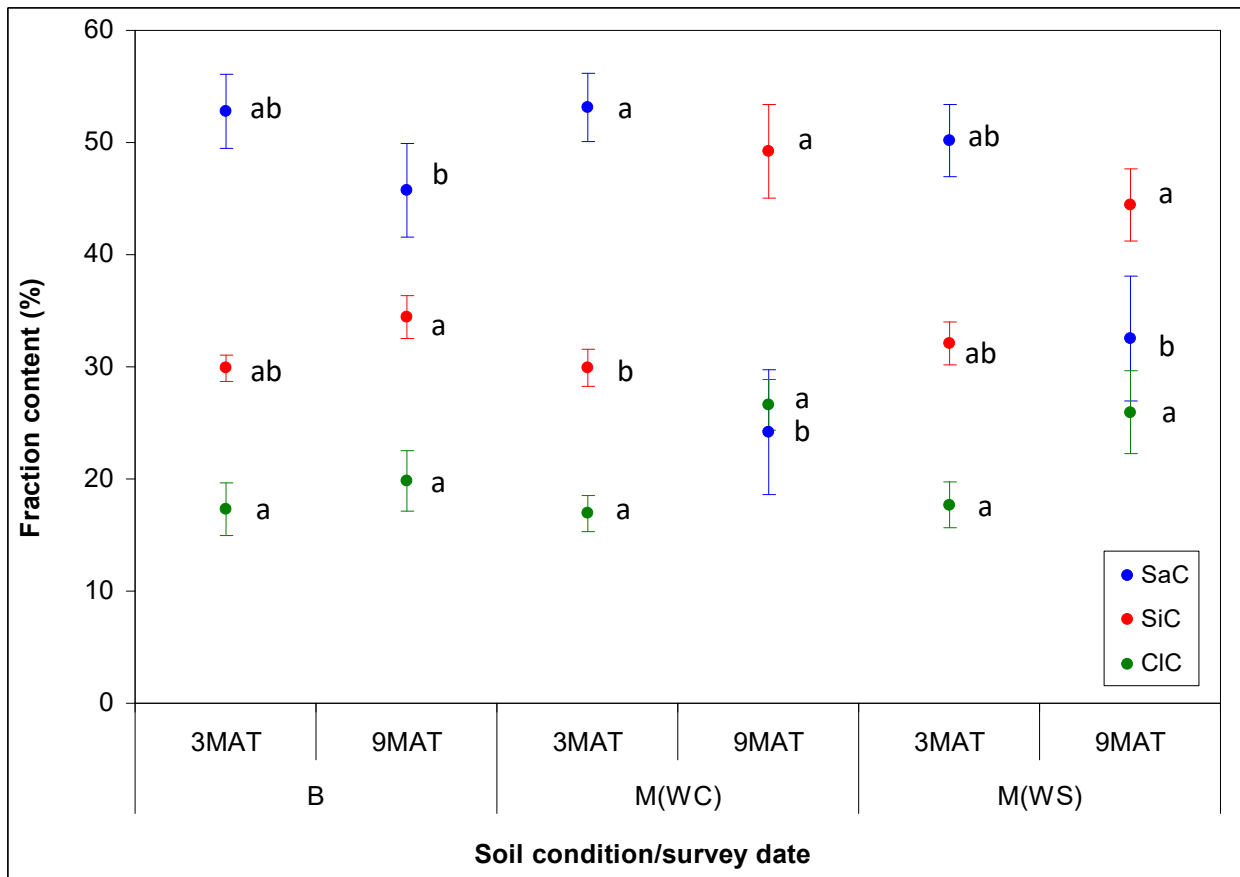
Figure 2 – Texture of samples of soils collected under three conditions (burned, B, mulched with wood chips, M(WC), and mulched with wheat straw, M(WS)) and two survey dates (at 3MAT and 9MAT) in Liétor (Castilla La Mancha, Central Eastern Spain). Legend: SaC = sand content; SiC = silt content; CIC = clay content. Different letters indicate significant differences in the interaction soil condition \times survey time after Tukey's test ( p < 0.05 ).
