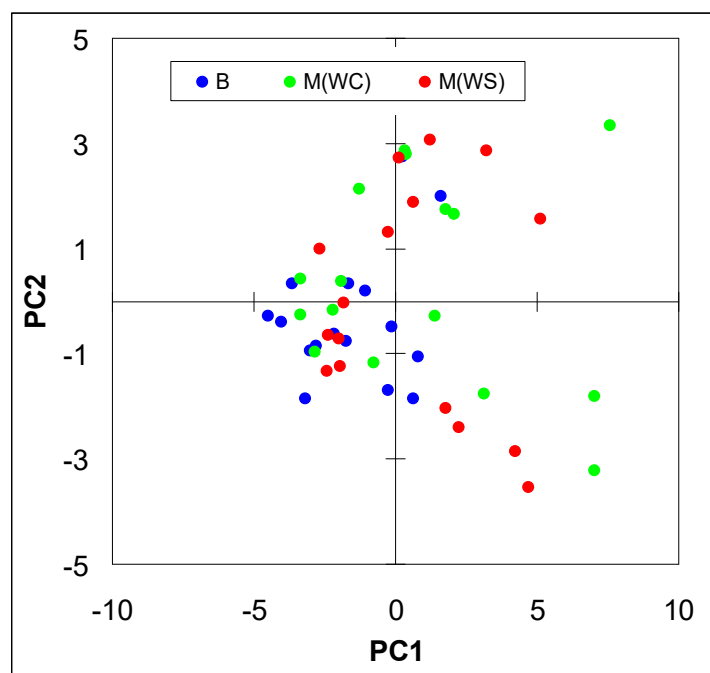
Figure 5 - Loadings of the original variables (main physico-chemical properties of soils) (a), and their scores on the first two Principal Components (PC1 and PC2) provided by PCA, applied to soil samples collected under three conditions (burned, B, mulched with wood chips, M(WC), and mulched with wheat straw, M(WS)) and two survey dates (at 3MAT and 9MAT) in Liétor (Castilla La Mancha, Spain). Legend: SaC = sand content; SiC = silt content; ClC = clay content; EC = electrical conductivity; OM = organic matter; TN = total nitrogen; N-NO 3 = nitric nitrogen; P = phosphorous; K = potassium; Na + = sodium; Ca 2+ = calcium; Mg 2+ = magnesium; Cl - = chloride; SO 4 2- = sulphates; CO 3 2- = carbonates; AL = active limestone.
