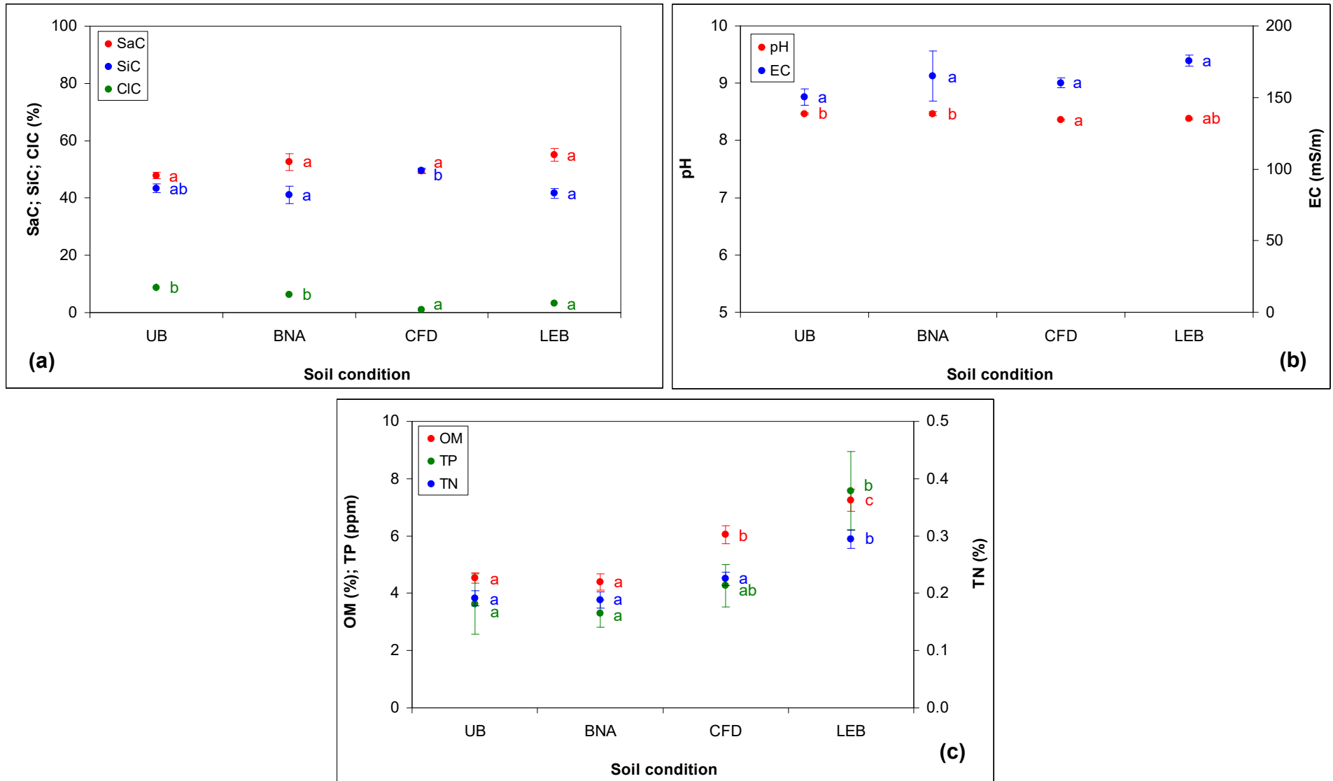
2 Figure 4 – Mean \pm standard error (n = 9 composite samples) of the main properties of soils under four soil conditions (UB = unburnt; BNA = burnt 3 and no action; CFD = contour felled log debris; LEB = log erosion barriers) six years after a wildfire in a semi-arid pine forest (Hellín, Castilla La
