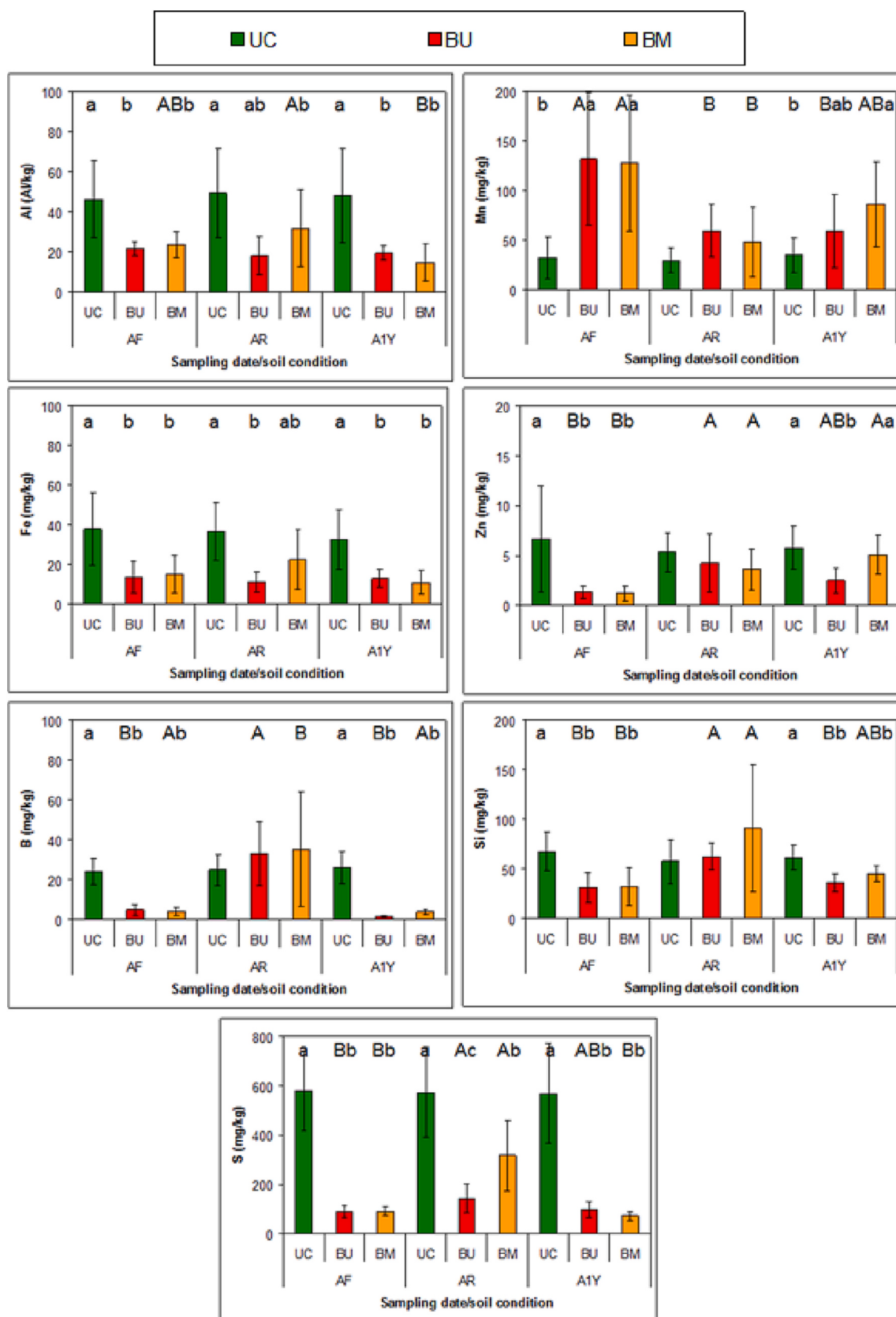
Fig. 5. Mean \pm standard deviation ( n = 9 ) for the minor extractable elements (Al, Mn, Fe, Zn, B, Si and S) under three soil conditions (UC, BU, BM) and on three sampling dates (AF, AR, A1Y) at a forest site (Braga, north-western Portugal). Note: Different letters represent significant differences at p < 0.05 among the sampling dates (capital letters) and soil conditions (lowercase letters).
