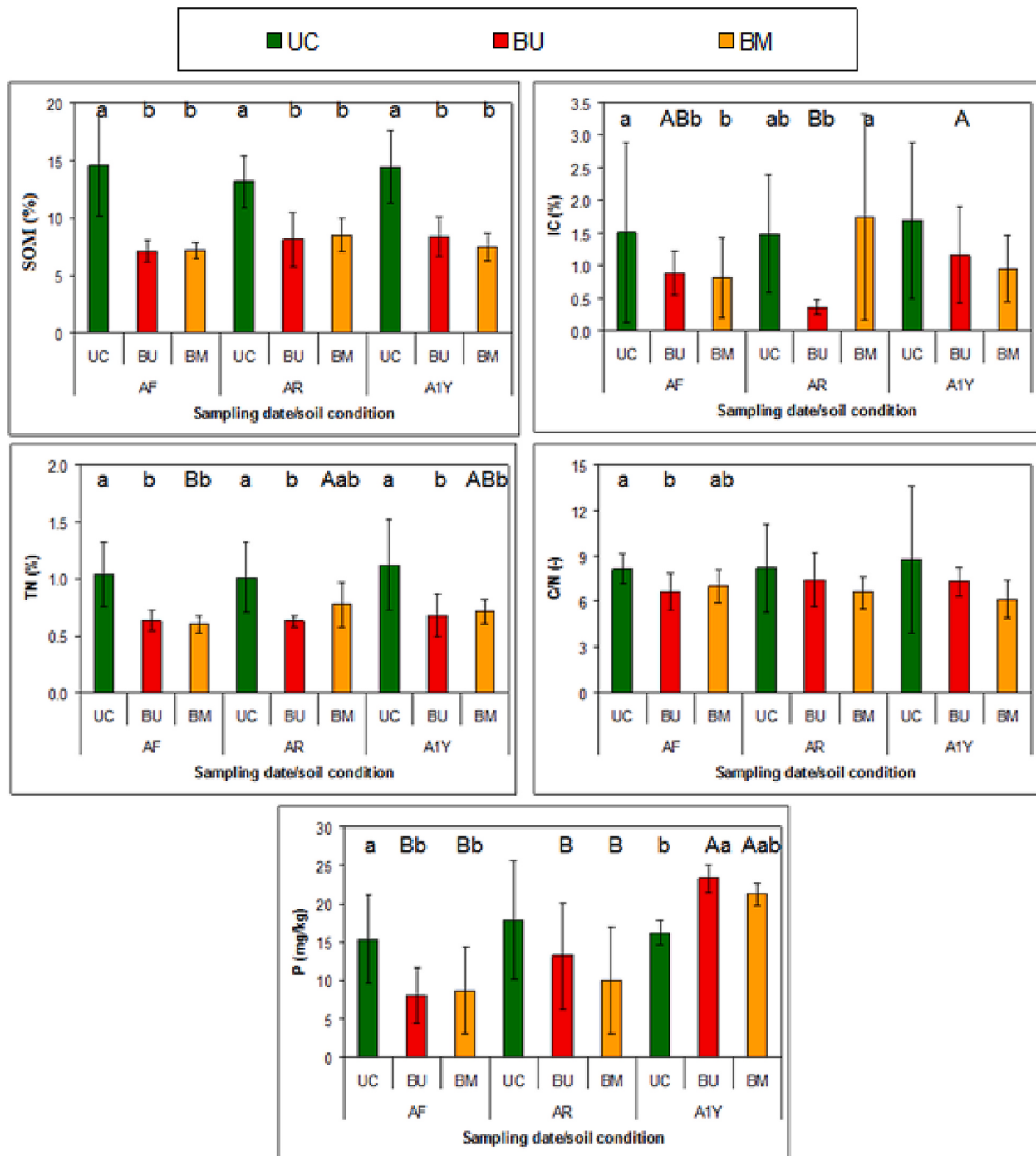
Fig. 3. Mean \pm standard deviation ( n = 9 ) for SOM, IC, TN, C:N ratio and available P under three soil conditions (UC, BU, BM) and on three sampling dates (AF, AR, A1Y) at a forest site (Braga, north-western Portugal). Note: Different letters represent significant differences at p < 0.05 among the sampling dates (capital letters) and soil conditions (lowercase letters).
