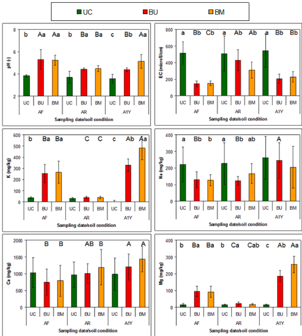
Fig. 4. Mean \pm standard deviation ( n = 9 ) for pH, EC and extractable cations (K, Na, Ca, Mg) under three soil conditions (UC, BU, BM) and on three sampling dates (AF, AR, A1Y) at a forest site (Braga, north-western Portugal). Note: Different letters represent significant differences at p < 0.05 among the sampling dates (capital letters) and soil conditions (lowercase letters).
