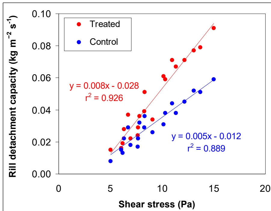
Figure 4 – Linear regression equations between the rill detachment capacity ( y = D_c ) and shear stress ( x = \tau ) estimated on soil samples collected in deforested hillslopes of Guilan province (Northern Iran) and treated with rice husk biochar or left undisturbed (control).
