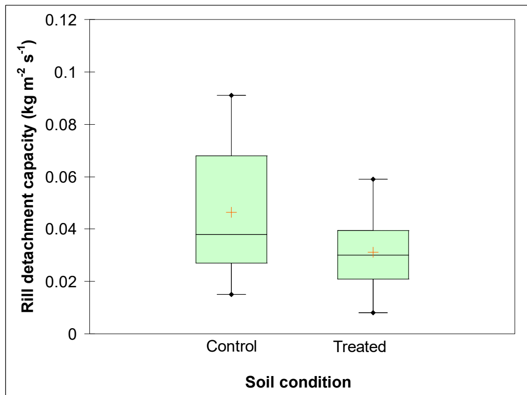
Figure 2 - Box plots of rill detachment capacity measured using flume experiments on samples collected in deforested hillslopes of Guilan province (Northern Iran) and treated with rice husk biochar or left undisturbed (control).
