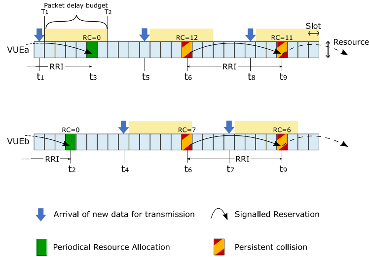
Fig. 1. Legacy SB-SPS. VUE a and VUE b perform a reselection at time t_5 and t_4 , respectively, due to RC = 0 . The two VUEs select the same resource and experience a collision at time t_6 . Since the allocation is performed with the same periodicity, the collision repeats at time t_9 and will repeat again at least until the RC of either VUE reaches 0.
