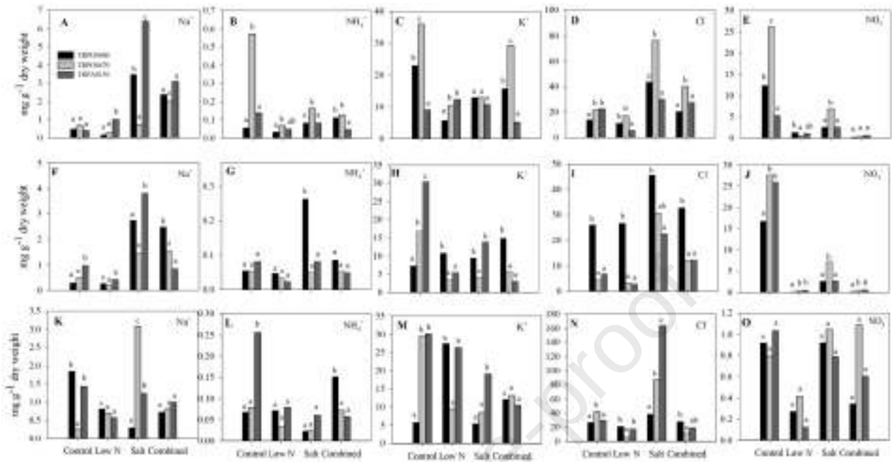
Figure 5. Ion content (mg g -1 Dry Weight) in leaf (A-E), stem (F-J) and fruit (K-O) of three tomato genotypes exposed to control, low N, salt stress and combined stress conditions. Different letters within treatments for each ion indicate means that differ significantly, according to Tukey's HSD test at p < 0.05 (n = 4).
