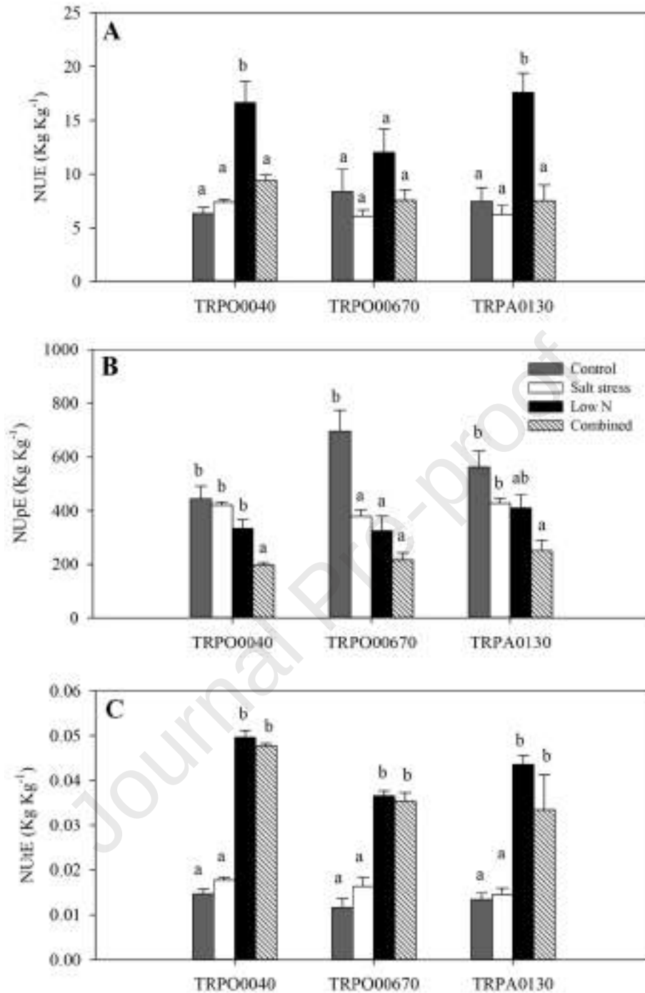
Figure 4. Nitrogen Use Efficiency (A), uptake efficiency (B) and utilization efficiency (C) of tomato genotypes TRPO0040, TRPO0670, and TRPA0130 exposed to control, low N, salt stress and combined stress conditions for 120 days. Different letters indicate significant differences at p < 0.05 according to Duncan post hoc test.
