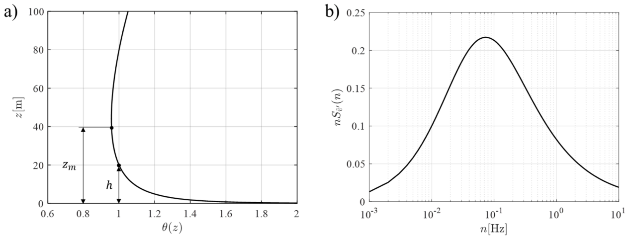
Fig. 2. (a) Vertical profile of the turbulence intensity \theta(z) and (b) PSD model of the turbulence S_v(z) .
