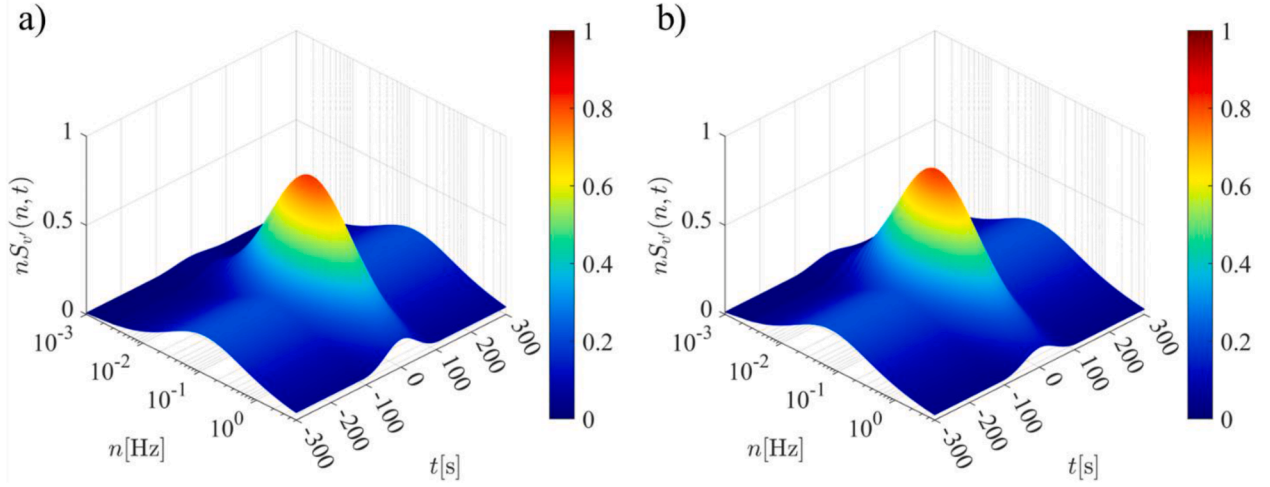
Fig. 25. Interval EPSD of the nonstationary turbulence v' evaluated for different values of the interval variables: (a) L_v^I = L_v, \gamma^{*I} = \gamma_0^*, T^I = T_0, z_m^I = z_{m,0}, I_v^I = I_{v,0} ; (b) L_v^I = L_v, \gamma^{*I} = \gamma_0^*, T^I = T_0, z_m^I = z_{m,0}, I_v^I = I_{v,0} .
