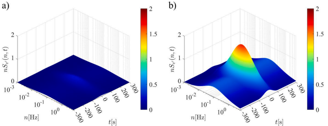
Fig. 26. Interval EPSD of the nonstationary turbulence v' evaluated for different values of the interval variables: (a) I_v^I = I_v, \gamma^{*I} = \gamma_0^*, T^I = T_0, z_m^I = z_{m,0}, L_v^I = L_{v,0} ; (b) I_v^I = I_v, \gamma^{*I} = \gamma_0^*, T^I = T_0, z_m^I = z_{m,0}, L_v^I = L_{v,0} .
