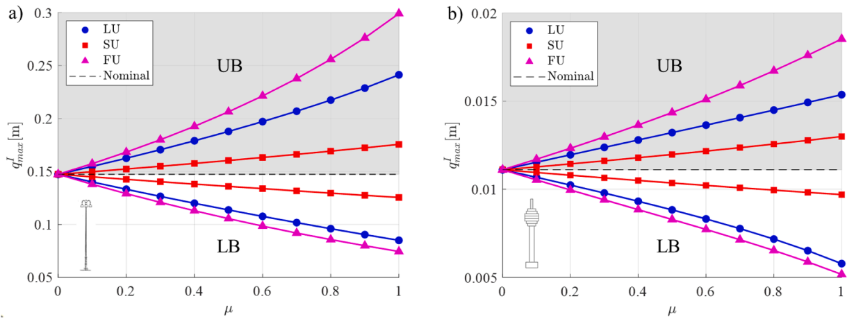
Fig. 19. Bounds of the maximum dynamic response for the (a) lighting pole and (b) telecommunications tower.
