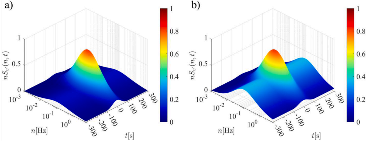
Fig. 22. Interval EPSD of the nonstationary turbulence v' evaluated for different values of the interval variables: (a) \gamma^{*I} = \gamma^* , T^I = T_0 , z_m^I = z_{m,0} , I_v^I = I_{v,0} , L_v^I = L_{v,0} ; (b) \gamma^{*I} = \bar{\gamma}^* , T^I = T_0 , z_m^I = z_{m,0} , I_v^I = I_{v,0} , L_v^I = L_{v,0} .
