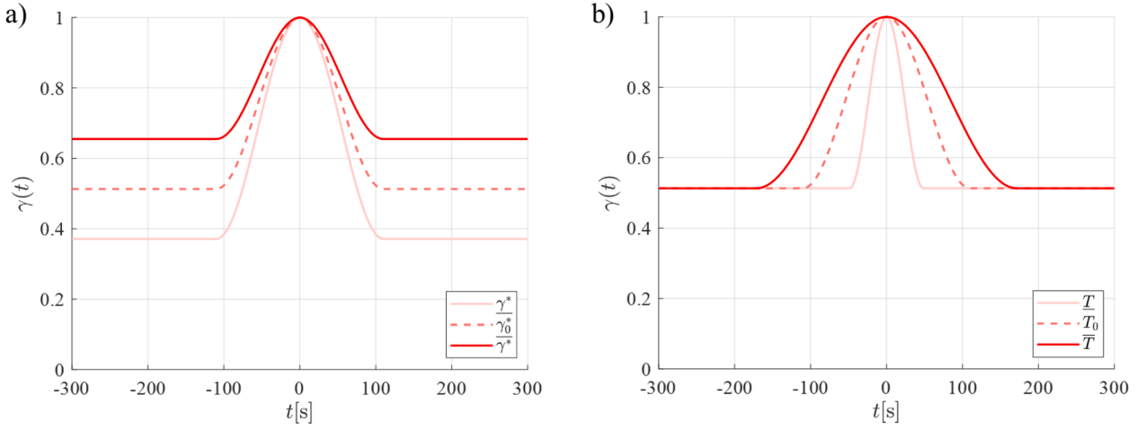
Fig. 5. Interval modulating function of the mean wind speed for different values of the interval variables: (a) T^I = T_0 , \gamma^{*I} = \underline{\gamma}^*, \gamma_0^*, \bar{\gamma}^* ; (b) \gamma^{*I} = \gamma_0^* , T^I = \underline{T}, T_0, \bar{T} .
