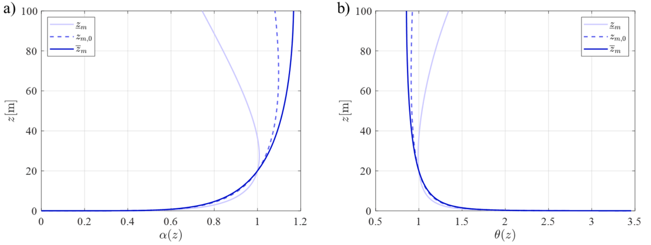
Fig. 6. (a) Interval vertical profile of the mean wind speed \alpha^I(z) and (b) turbulent intensity \theta^I(z) for z_m^I = \underline{z}_m, z_{m,0}, \bar{z}_m .
