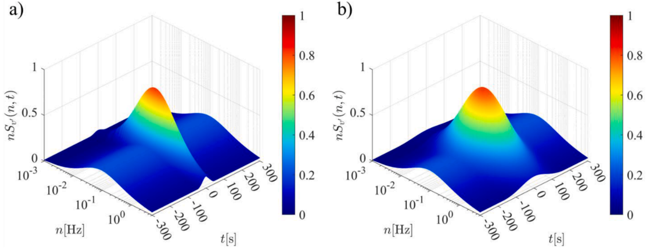
Fig. 23. Interval EPSD of the nonstationary turbulence v' evaluated for different values of the interval variables: (a) T^I = \underline{T} , \gamma^{*I} = \gamma_0^* , z_m^I = z_{m,0} , I_v^I = I_{v,0} , L_v^I = L_{v,0} ; (b) T^I = \bar{T} , \gamma^{*I} = \gamma_0^* , z_m^I = z_{m,0} , I_v^I = I_{v,0} , L_v^I = L_{v,0} .
