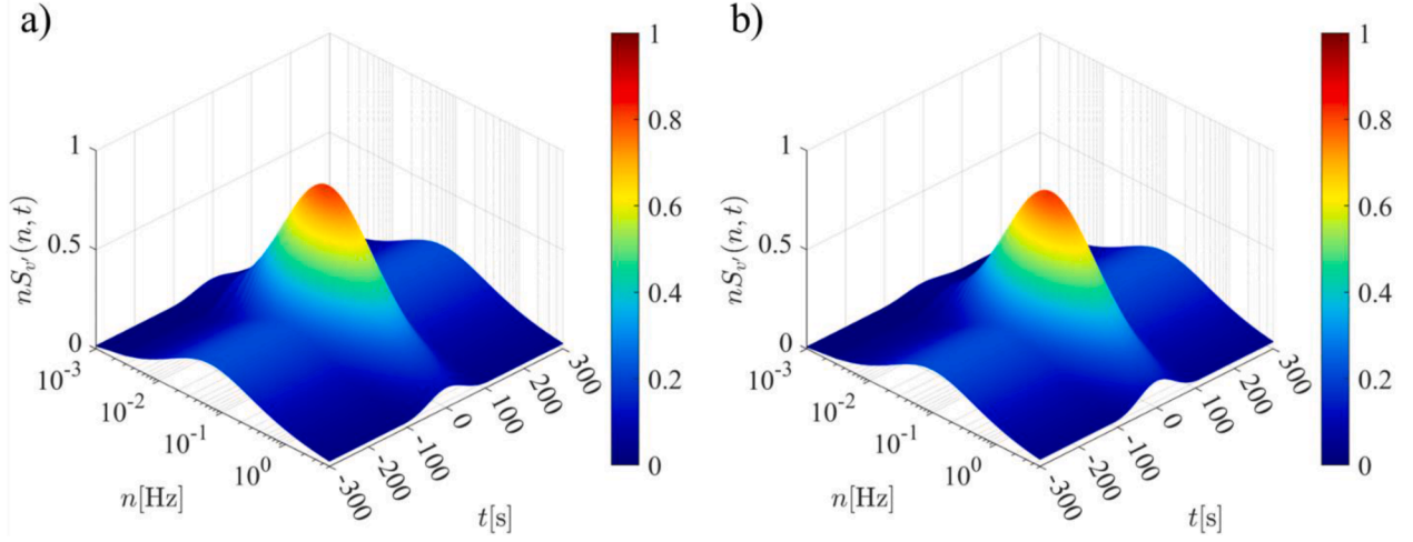
Fig. 24. Interval EPSD of the nonstationary turbulence v' evaluated for different values of the interval variables: (a) z_m^I = z_m, \gamma^{*I} = \gamma_0^*, T^I = T_0, I_v^I = I_{v,0}, L_v^I = L_{v,0} ; (b) z_m^I = z_m, \gamma^{*I} = \gamma_0^*, T^I = T_0, I_v^I = I_{v,0}, L_v^I = L_{v,0} .
