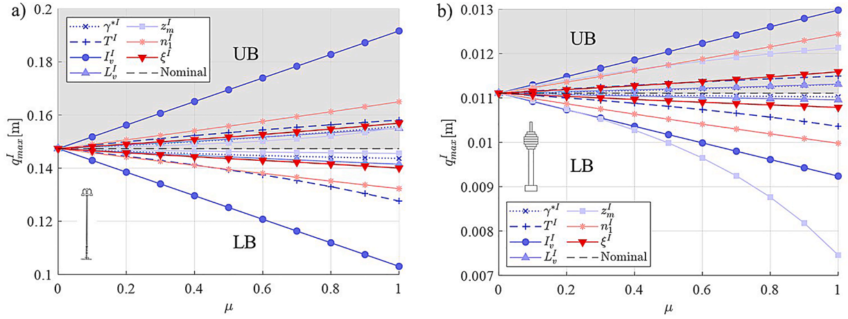
Fig. 17. LB and UB of the maximum response estimated considering one interval parameter at a time: (a) case study 1; (b) case study 2.
