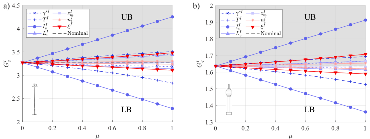
Fig. 16. LB and UB of the TGRF estimated considering one interval parameter at a time: (a) case study 1; (b) case study 2.
