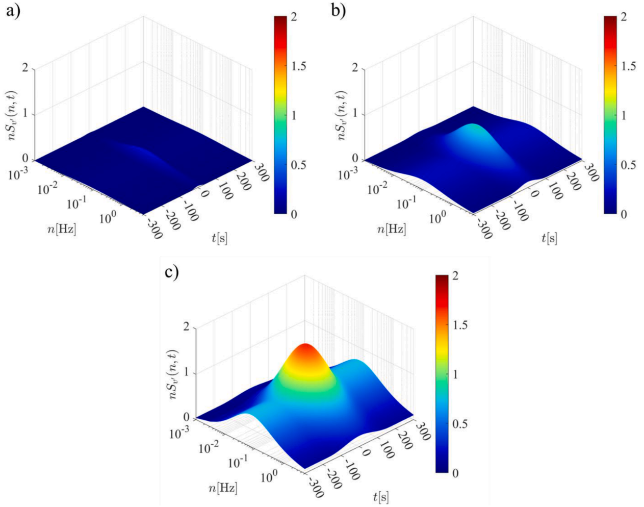
Fig. 8. Interval EPSD of the nonstationary turbulence v' evaluated for different values of the interval variables: (a) \mathbf{x}_L^I = \underline{\mathbf{x}}_L ; (b) \mathbf{x}_L^I = \mathbf{x}_{L,0} ; (c) \mathbf{x}_L^I = \bar{\mathbf{x}}_L .
