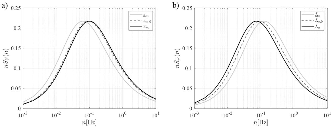
Fig. 7. Interval PSD function of the reduced fluctuations for different values of the interval variables: (a) L_v^I = L_{v,0}, z_m^I = \underline{z}_m, z_{m,0}, \bar{z}_m ; (b) z_m^I = z_{m,0}, L_v^I = \underline{L}_v, L_{v,0}, \bar{L}_v .
