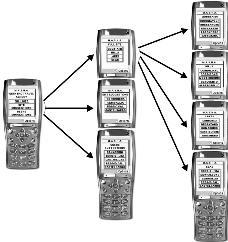
Figure 5. The mobile presentation of a MASHA Web travel agency.
