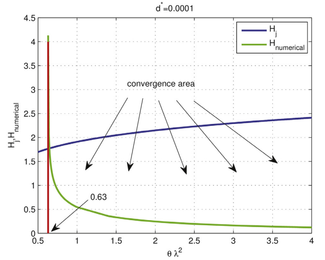
Fig. 1. Convergence area achieved in [3] with d^* = 0.0001 .
