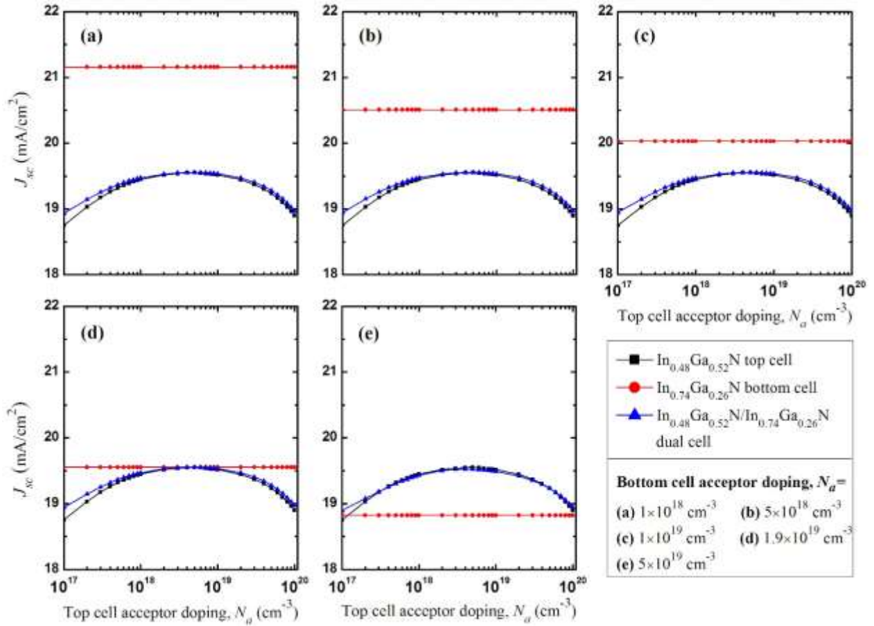
Fig. 5. J_{sc} as a function of the top cell acceptor concentration for different values of N_a in the bottom cell. In each sub-cell N_a/N_d=10^3 , d_B = 1 \mu\text{m} , and d_E = 0.01 \mu\text{m} .
