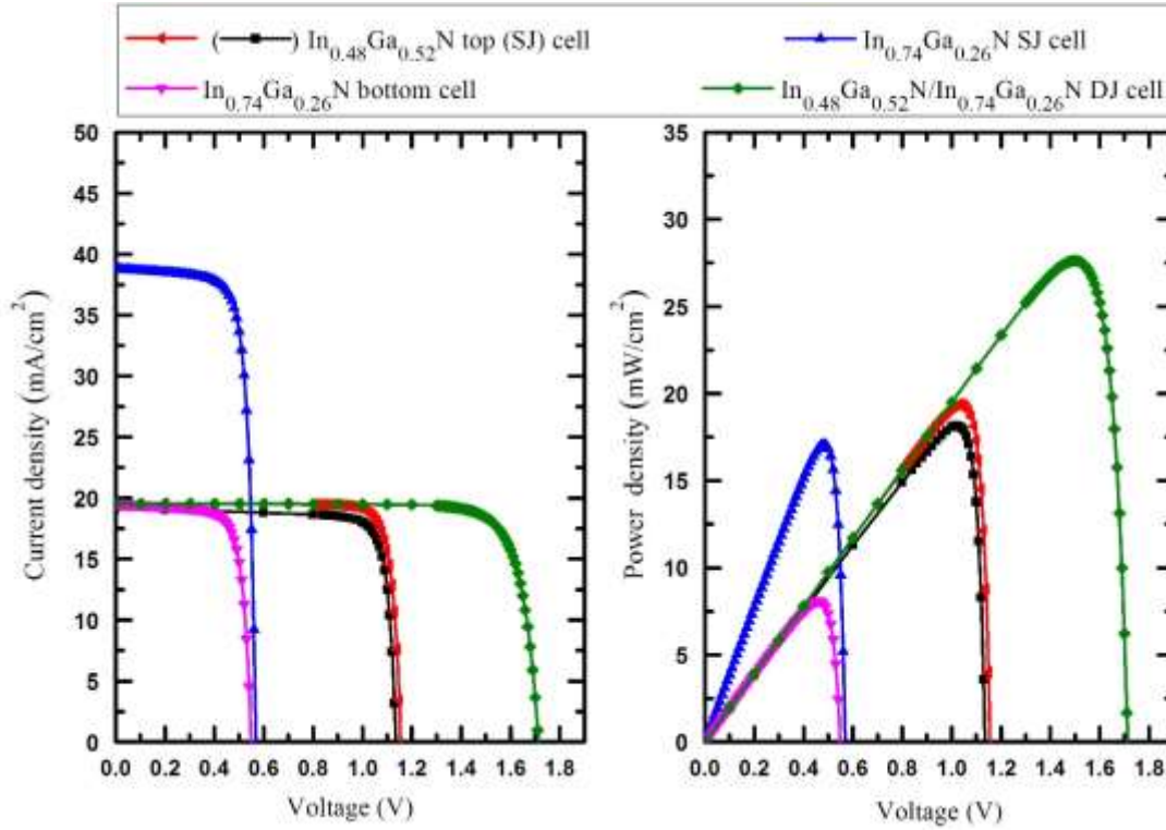
Fig. 9. (a) J - V and (b) P - V characteristics.
