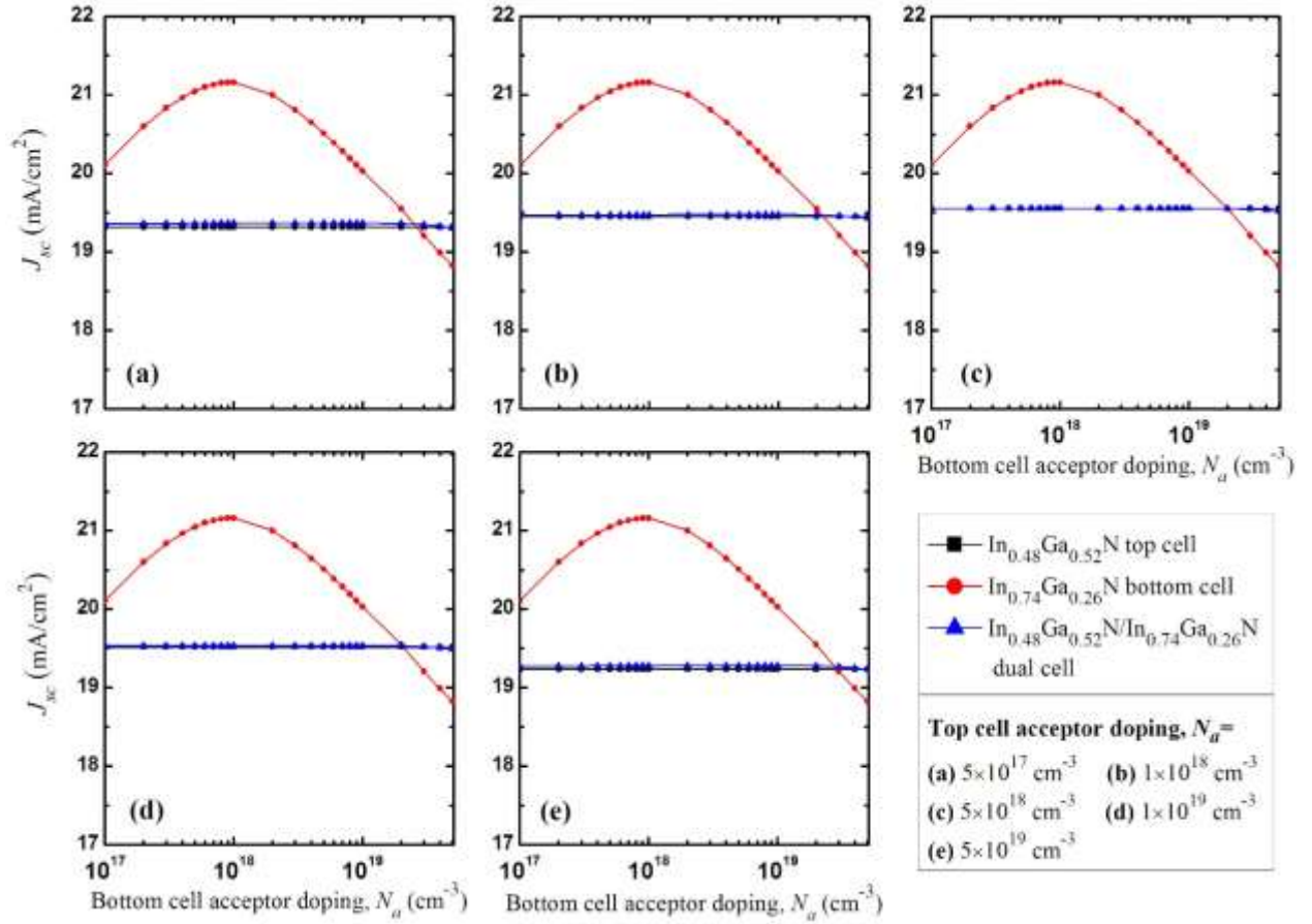
Fig. 6. J_{sc} as a function of the bottom cell acceptor concentration for different values of N_a in the top cell. In each sub-cell N_a/N_d=10^3 , d_B = 1 \mu\text{m} and d_E = 0.01 \mu\text{m} .
