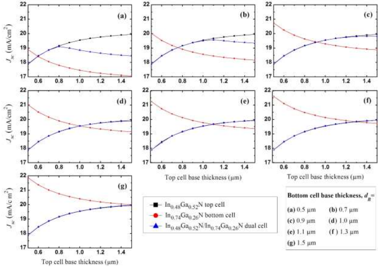
Fig. 7. J_{sc} as a function of the top cell base thickness for different values of d_B in the bottom cell. N_{a(top)} = 5 \times 10^{18} \text{ cm}^{-3} , N_{a(bot)} = 1.9 \times 10^{19} \text{ cm}^{-3} , and d_E = 0.01 \text{ } \mu\text{m} in each sub-cell.
