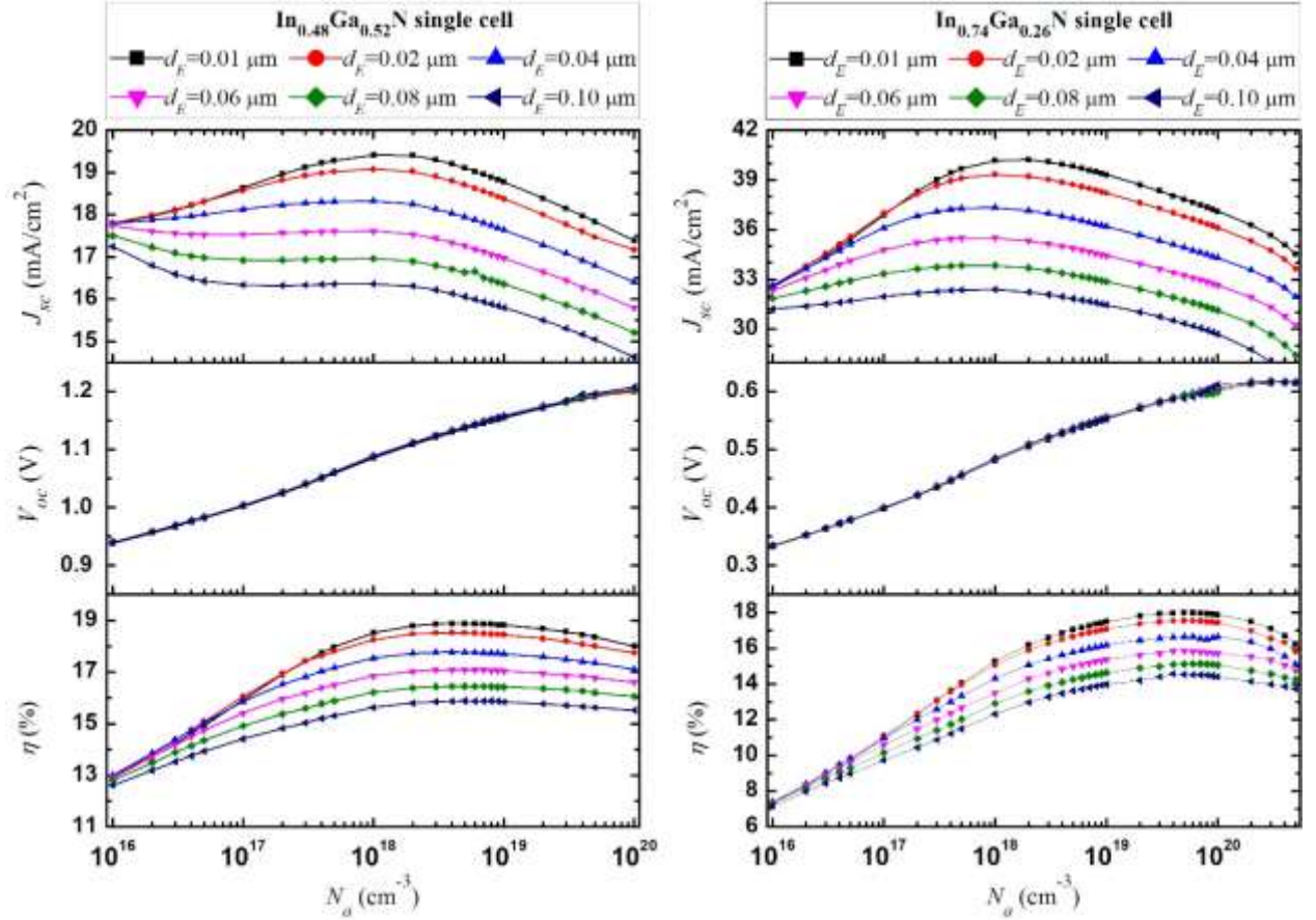
Fig. 2. Short-circuit current density J_{sc} , open-circuit voltage V_{oc} , and conversion efficiency \eta for the top and bottom single cell in Fig. 1. A doping concentration ratio N_a/N_d = 10^3 was imposed during the simulations and d_B = 1 \mu\text{m} .
