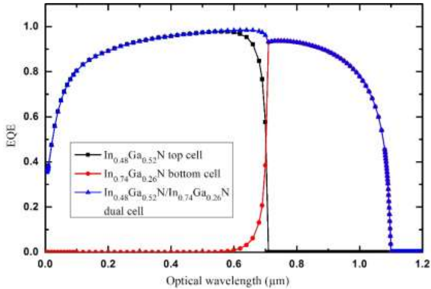
Fig. 8. External quantum efficiency of the top, bottom, and dual cell design.
