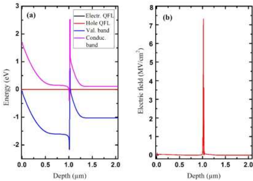
Fig. 4. (a) Energy band diagram. (b) Electric field profile.
