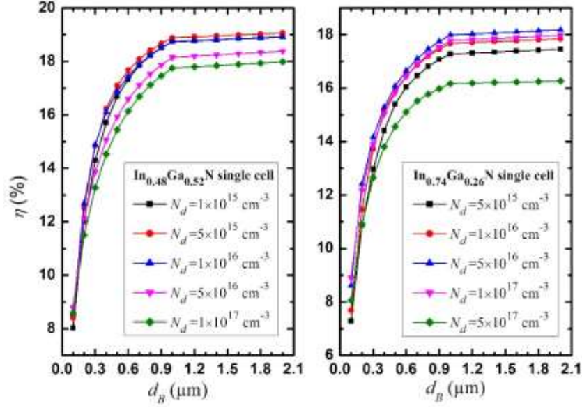
Fig. 3. Conversion efficiency as a function of the base thickness for different values of the donor doping concentration. N_a/N_d=10^3 and d_E = 0.01 \mu\text{m} .
