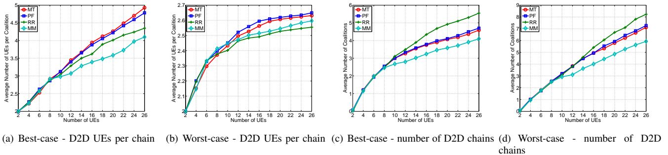
Fig. 6. Configuration of multihop D2D chains as a result of the coalition formation game.
