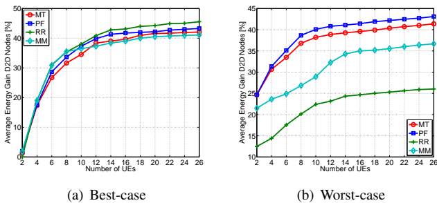
Fig. 7. Average energy consumption gain for UEs in the D2D chain.
