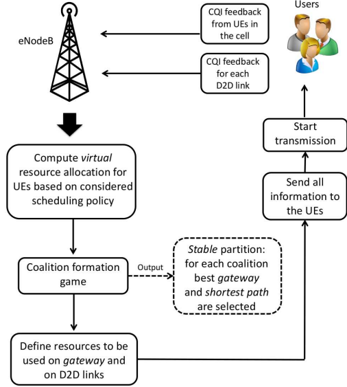
Fig. 2. Flowchart of the proposed solution.
