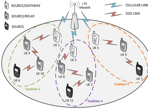
Fig. 1. Multihop D2D-based content uploading.
