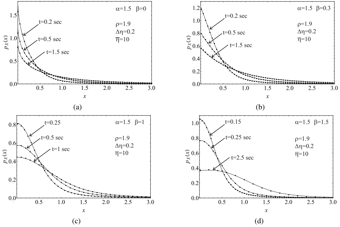
Figure 2: CFM solution (continuous line) versus PDF by digital simulation (dotted curves) for \alpha = 1.5 at various instant and for different \beta .
