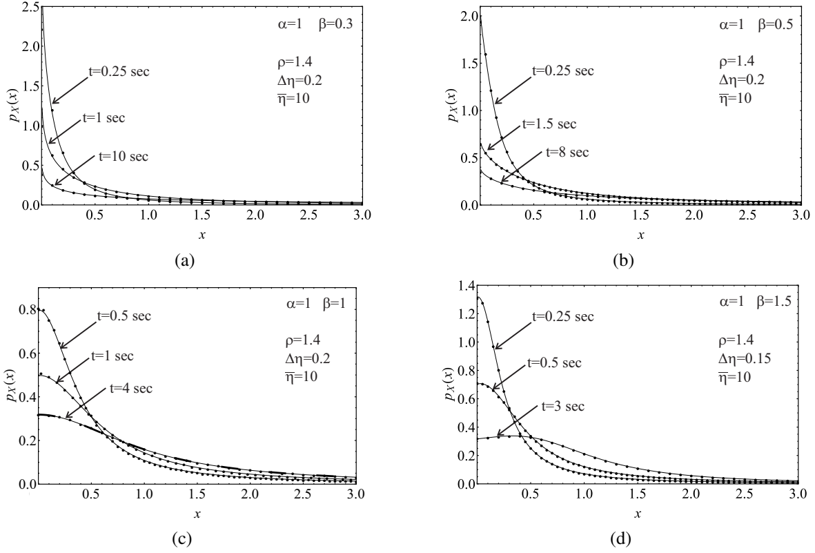
Figure 3: CFM solution (continuous line) versus PDF by digital simulation (dotted curves) for \alpha = 1 at various instant and for different \beta .
