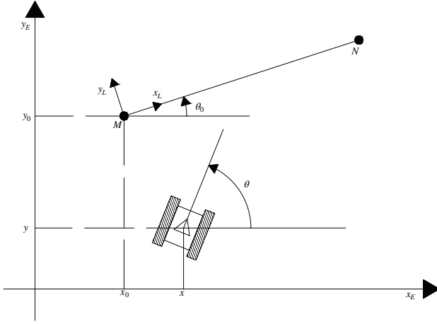
Fig. 1. Coordinate Frames for the skid-steering tracked robot.
