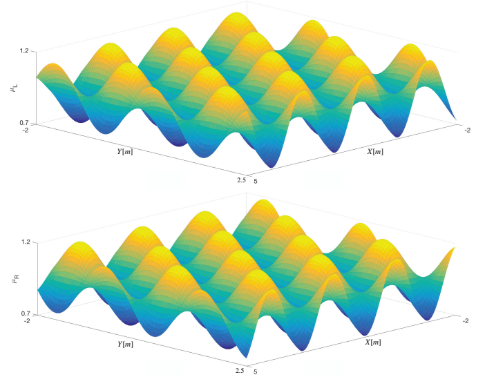
Fig. 7. Friction coefficients.
