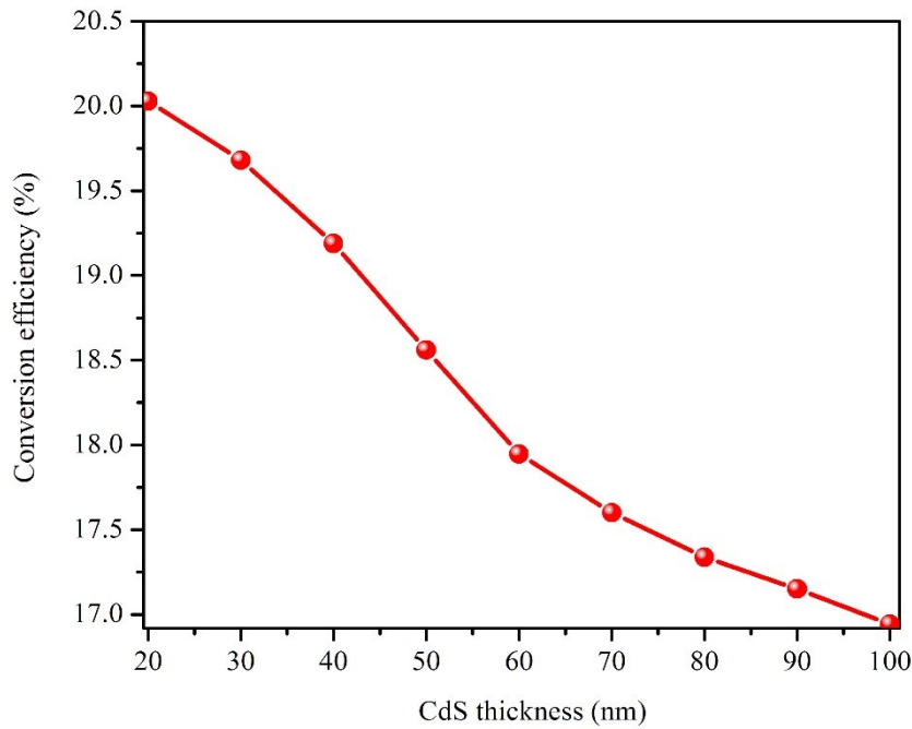
Fig. 6. Cell efficiency as a function of the CdS layer thickness.
