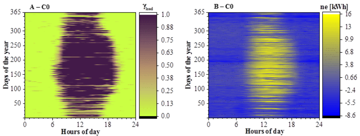
Fig. 4. Coloured contour graph of the \gamma_{load} (A) and ne (B) for the first year in the C0.
