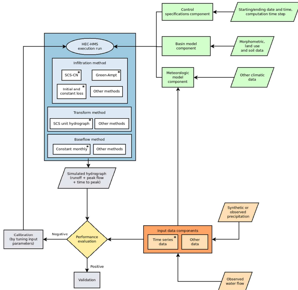
Figure 3 – HEC-HMS model structure and evaluation procedure (the symbol * indicates the method/component used in this work).
