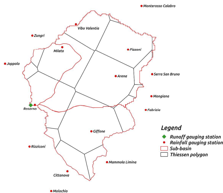
Figure 4 – Rainfall and water level gauging stations as well as Thiessen's polygons in the Mésima torrent (Calabria, Southern Italy).
