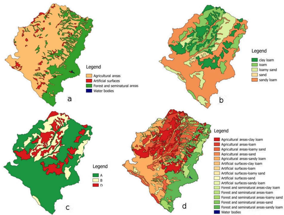
Figure 2 – Maps of land use (a, from Corine Land Cover, 2007), texture (b, ARSSA, 2003), hydrologic group (c) and homogenous hydrological units (HRU, d) in the Mésima torrent (Calabria, Southern Italy).
