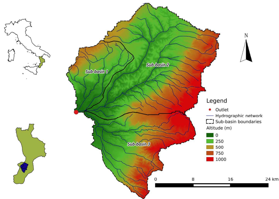
Figure 1 - Location and Digital Elevation Model of the Mésima torrent (Calabria, Southern Italy).
