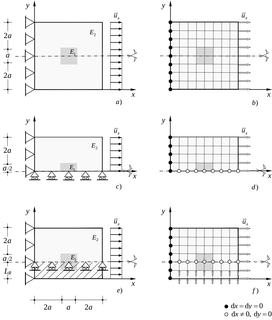
Fig. 1. Nonlocal elastic symmetric square plate under tension with piecewise constant Young modulus. Mechanical model of: a) whole structure; c) symmetric half structure; e) enlarged symmetric half structure. b), d) and f) FE models of structures a), c) and e), respectively.
