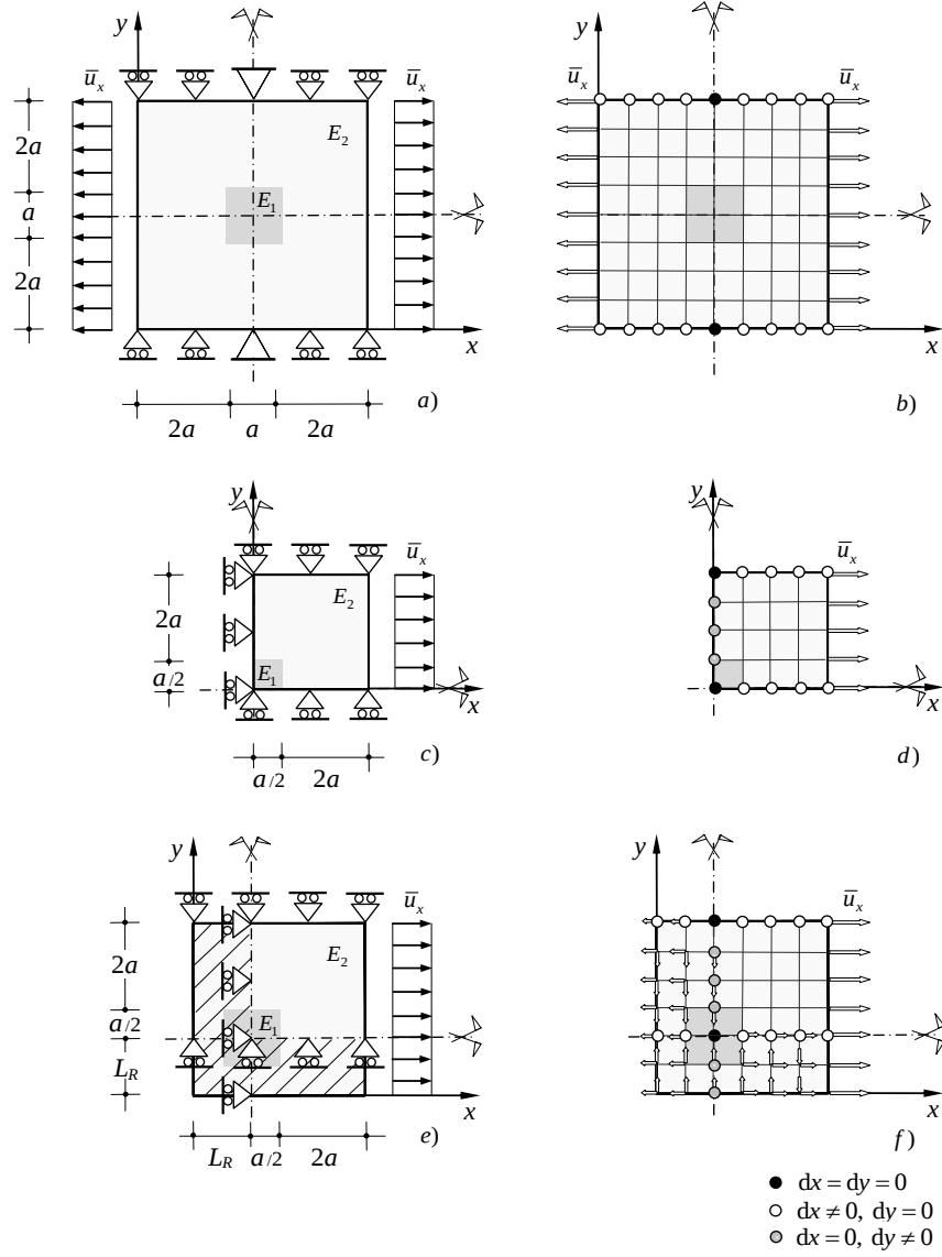
Fig. 4. Nonlocal elastic bi-symmetric square plate under tension with piecewise constant Young modulus. Mechanical model of: a) whole structure; c) symmetric quarter structure; e) enlarged symmetric quarter structure. b), d) and f) FE models of structures a), c) and e), respectively.
