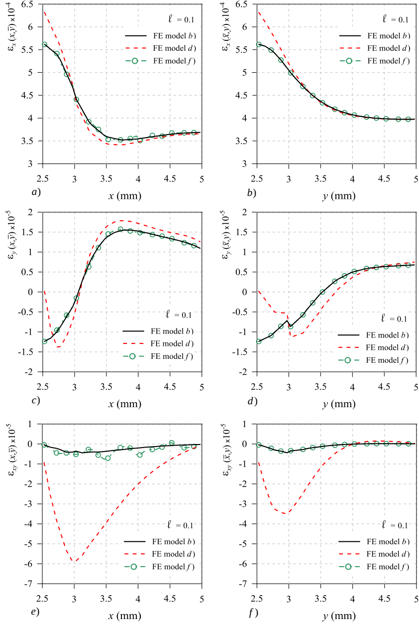
Fig. 5. Nonlocal elastic bi-symmetric square plate ( \ell = 0.1\text{cm} ). Strain components profiles \varepsilon_x , \varepsilon_y , \varepsilon_{xy} , versus x at y \simeq 2.5 on the left side and versus y at x \simeq 2.5 on the right side. Solution referred to the entire plate (solid lines), solution referred to the quarter symmetric portion (dashed lines), solution referred to the enlarged quarter symmetric portion (dashed lines with circles).
