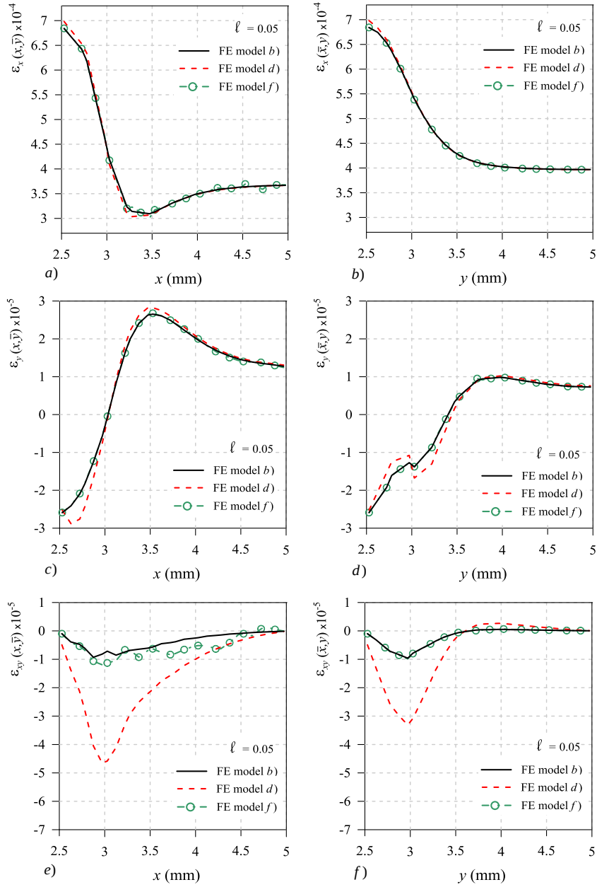
Fig. 6. Nonlocal elastic bi-symmetric square plate ( \ell = 0.05\text{cm} ). Strain components profiles \varepsilon_x , \varepsilon_y , \varepsilon_{xy} , versus x at y \simeq 2.5 on the left side and versus y at x \simeq 2.5 on the right side. Solution referred to the entire plate (solid lines), solution referred to the quarter symmetric portion (dashed lines), solution referred to the enlarged quarter symmetric portion (dashed lines with circles).
