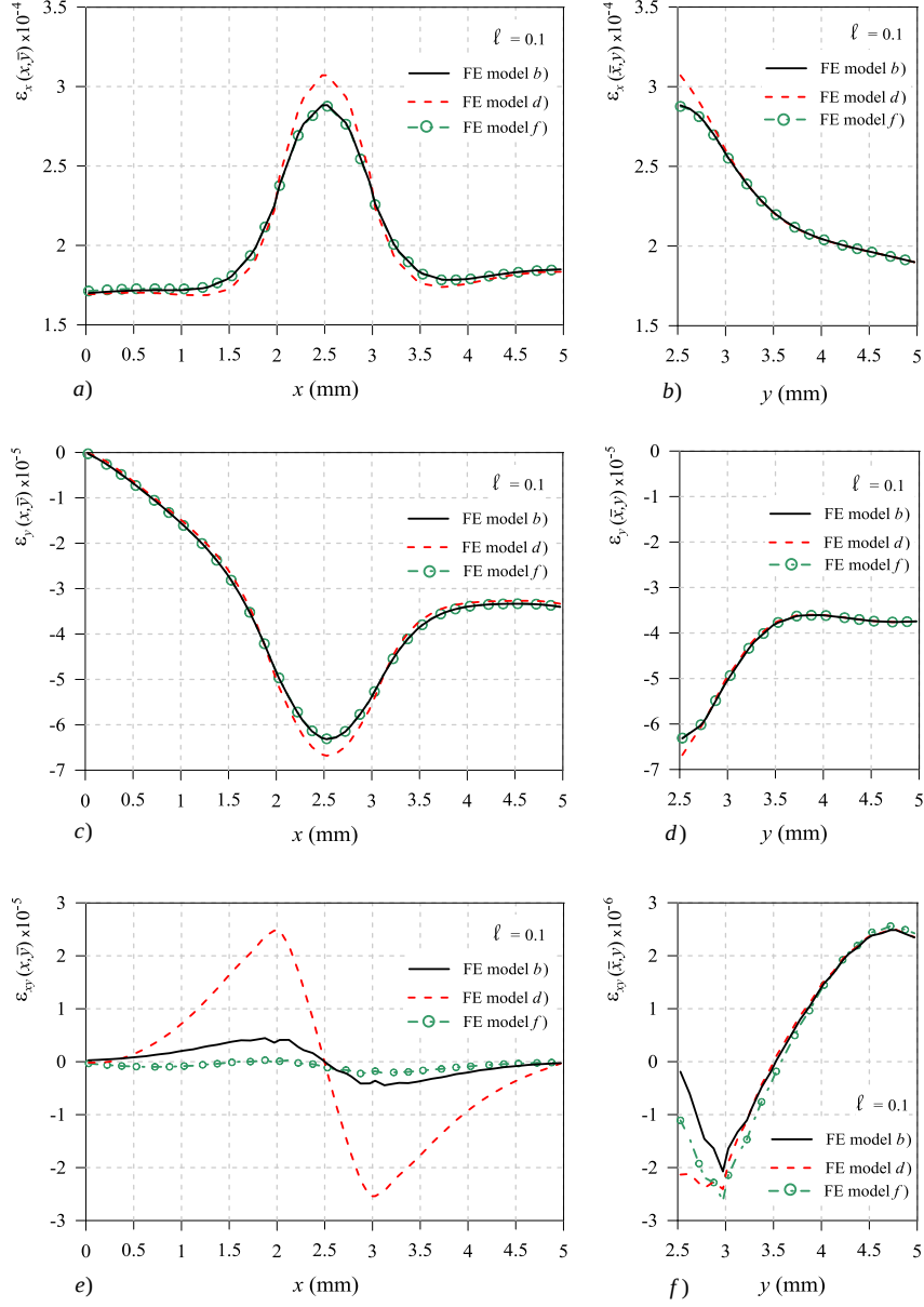
Fig. 2. Nonlocal elastic symmetric square plate ( \ell = 0.1 cm). Strain components profiles \varepsilon_x , \varepsilon_y , \varepsilon_{xy} , versus x at y = 2.5 on the left side and versus y at x = 2.5 on the right side. Solution referred to the entire plate (solid lines), solution referred to the half symmetric portion (dashed lines), solution referred to the enlarged half symmetric portion (dashed lines with circles).
