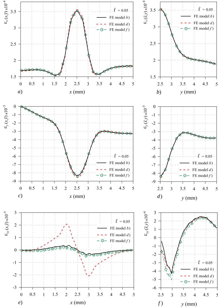
Fig. 3. Nonlocal elastic symmetric square plate ( \ell = 0.05 cm). Strain components profiles \varepsilon_x , \varepsilon_y , \varepsilon_{xy} , versus x at y \simeq 2.5 on the left side and versus y at x \simeq 2.5 on the right side. Solution referred to the entire plate (solid lines), solution referred to the half symmetric portion (dashed lines), solution referred to the enlarged half symmetric portion (dashed lines with circles).
