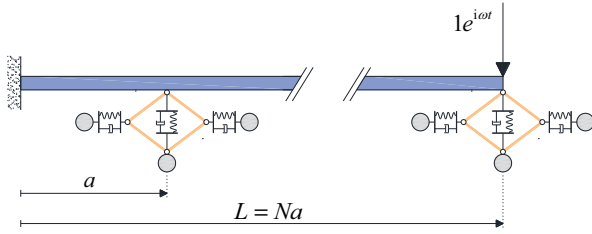
Fig. 3. Elastic LR beam with resonators in Fig. 2c.
