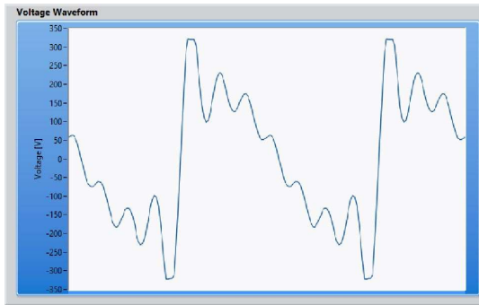
Fig. 7. Voltage waveform.
