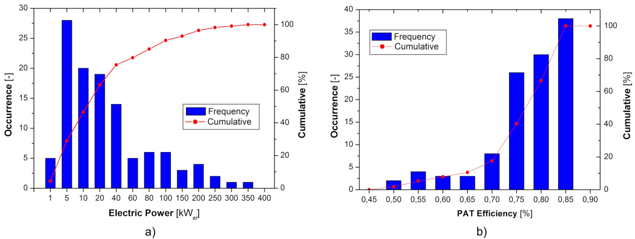
Figure 10 – Cumulative and frequency distribution of HP nominal electric power (a) and PAT efficiency (b).
