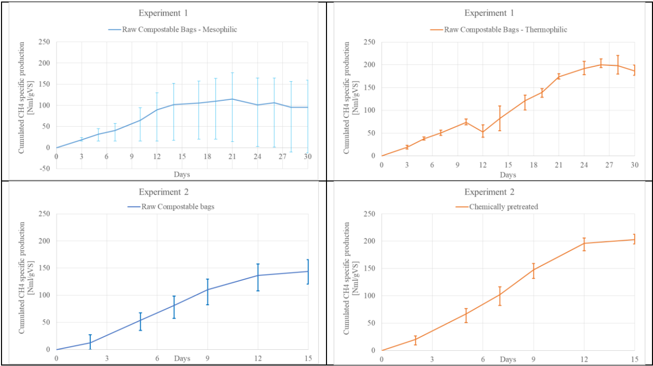
256 Figure 1. Cumulative methane production for some of the batch tests 257
