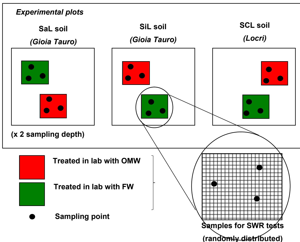
Figure 1 - Geographic location of the investigated olive groves (a) and experimental design for the SWR tests (b).
