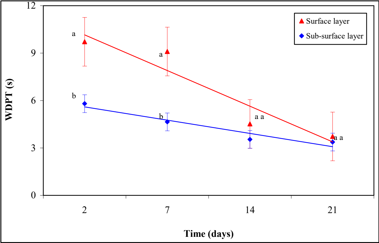
332 333 Figure 3 - Interactions between soil depth and time factors of three-way ANOVA applied to SWR 334 tests (WDPT = water drop penetration test) (different letters indicate significant differences after 335 Tukey's test ( p < 0.001 ).
