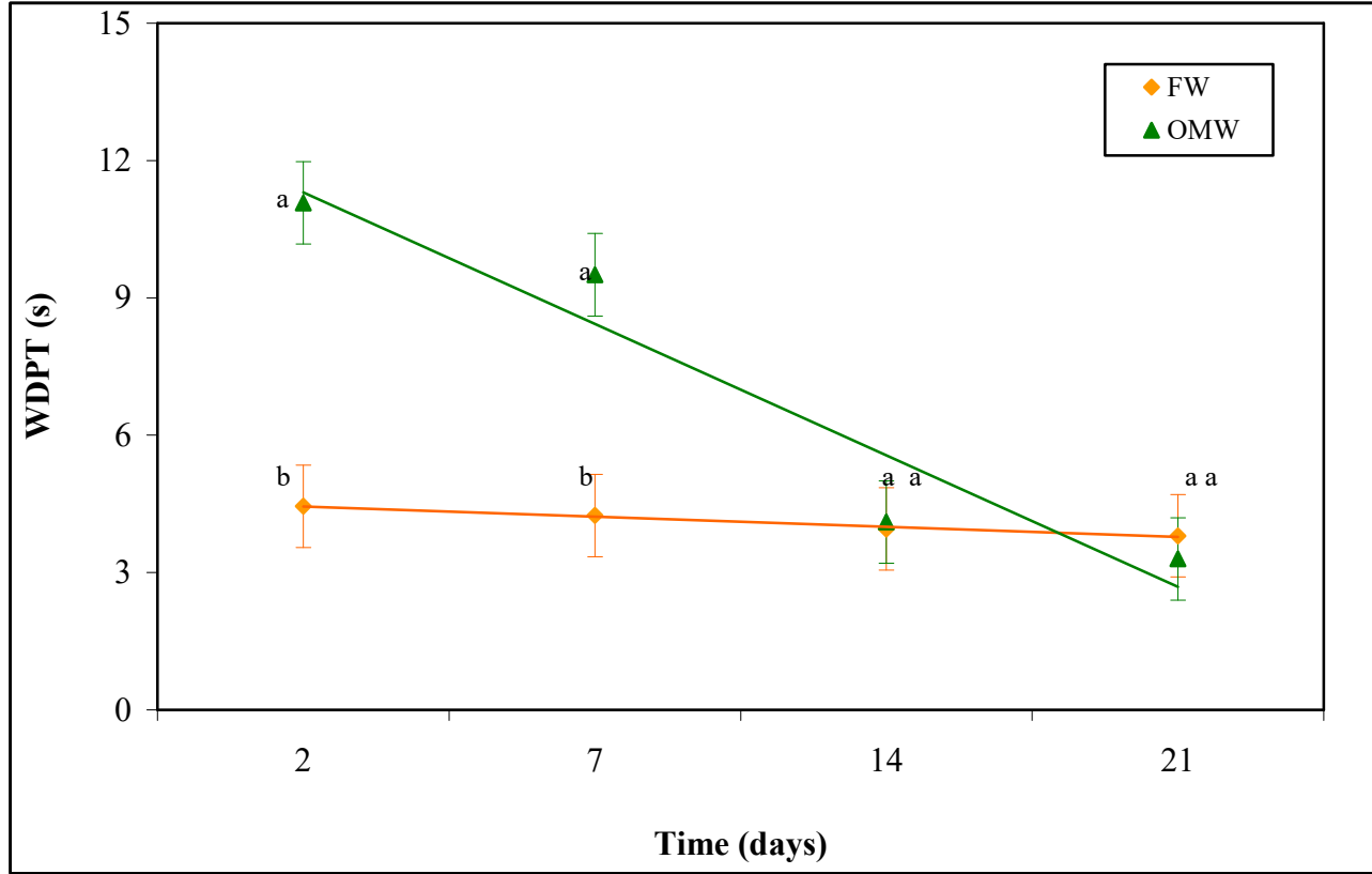
Figure 2 - Interactions between treatment and time factors of three-way ANOVA applied to SWR tests (WDPT = water drop penetration test) (different letters indicate significant differences after Tukey's test ( p < 0.001 )).
