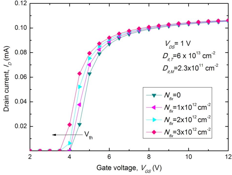
Figure. 11. Oxide fixed traps effect on the I_D - V_{GS} curves of an HfO 2 /4H-SiC MOSFET
