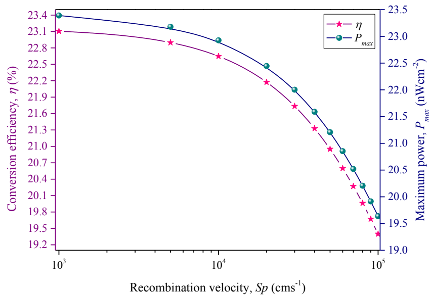
Fig. 5 Evolution of \eta and P_{max} as a function of S_p .
