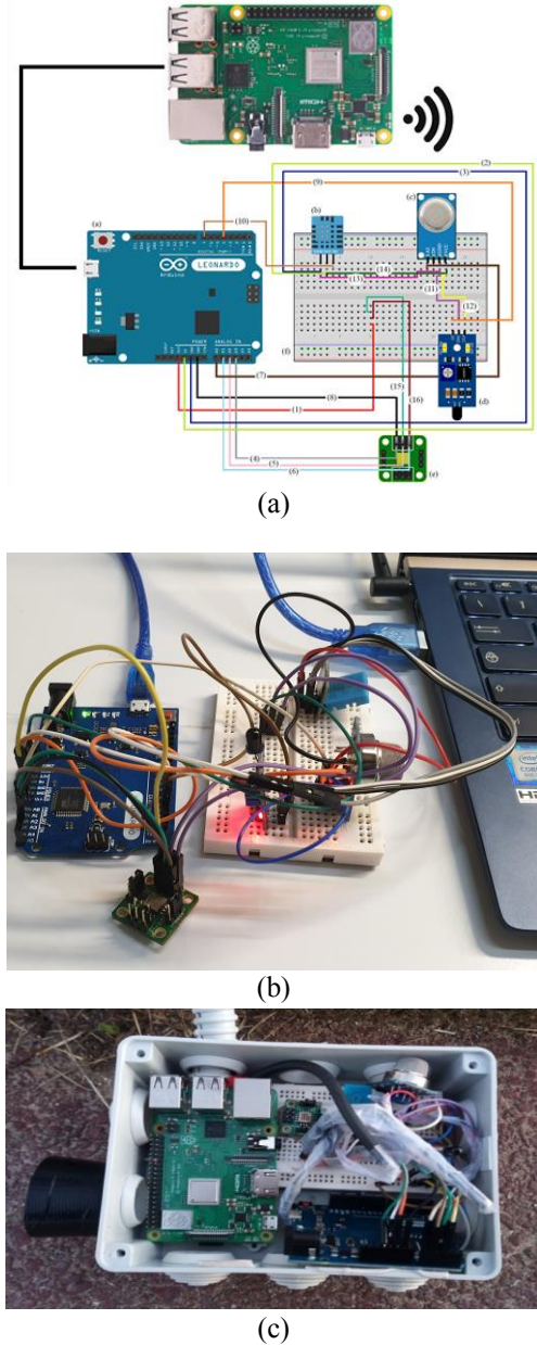
Fig. 1. Wireless sensor unit: a) first prototype; b) prototype during in-lab tests; c) first prototype during on site tests.
