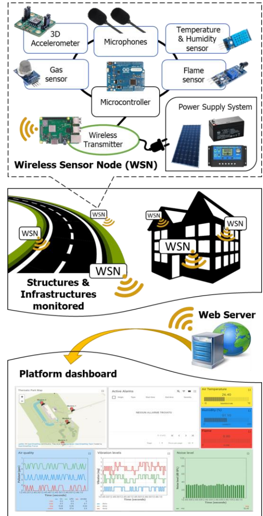
Fig. 3. Schematic representation of the monitoring platform.
