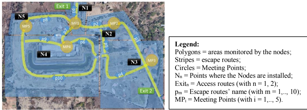
Fig. 6. Graph that shows the position of the nodes of the platform, of the escape routes, of the meeting points, and the areas monitored by each IoT node.
