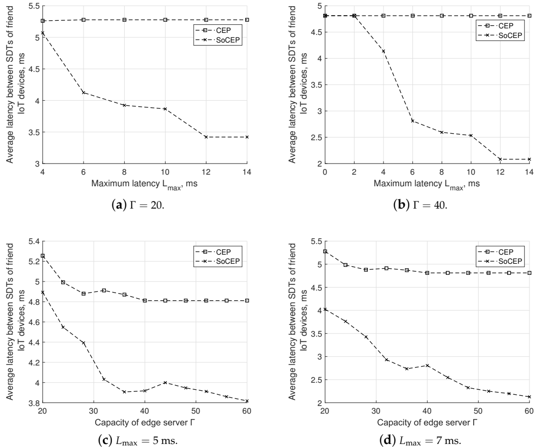
Figure 5. SoCEP vs. CEP: average latency between SDTs of friend IoT devices.
