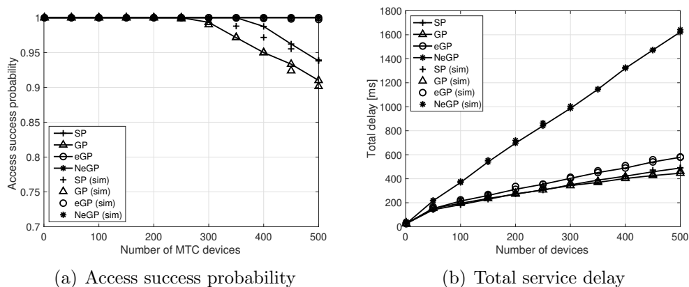
Figure 9: Access success probability and total service delay (small payload).
