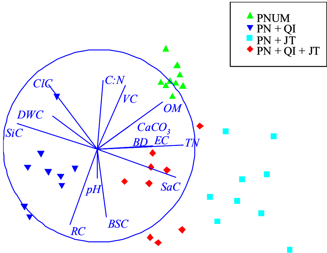
Figure 2 - Biplot of physico-chemical properties and covers of soil samples collected in plots under four tree diversity levels using nonmetric multidimensional scaling (NMDS) routine (Los Palancares y Agregados, Castilla-La Mancha, Spain). The stress value for the NMDS is 0.09. See the related list for the abbreviations.
