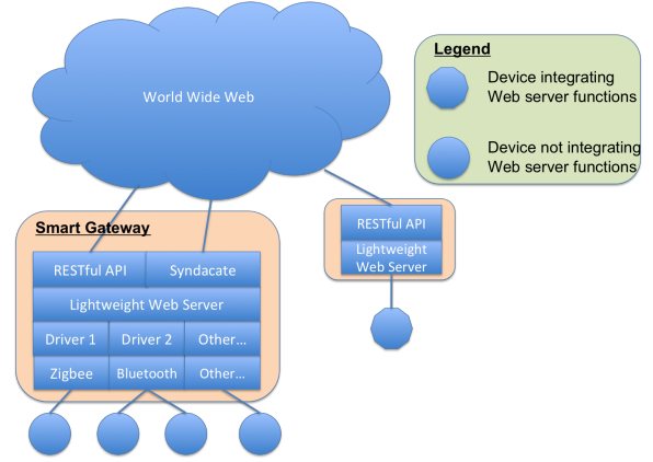
Fig. 7. Architecture of the Web of Things.
