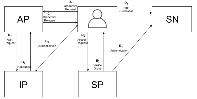
Fig. 1. Conceptual overview of our solution.
