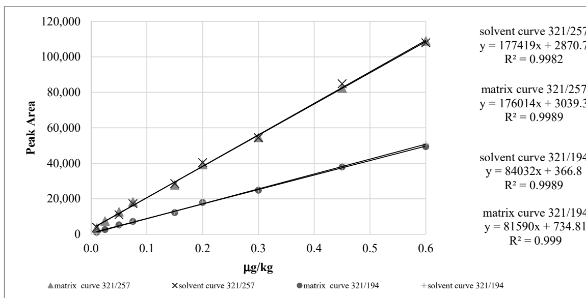
Figure 3. Comparison between calibration curve in solvent and in matrix at the same concentration range for 321→257 and 321→194 ion transitions.
