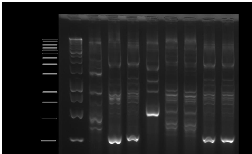
Fig. 4: BOX-PCR profile of 9 selected bacteria strains. Lane M denotes 1 kb DNA ladders.
