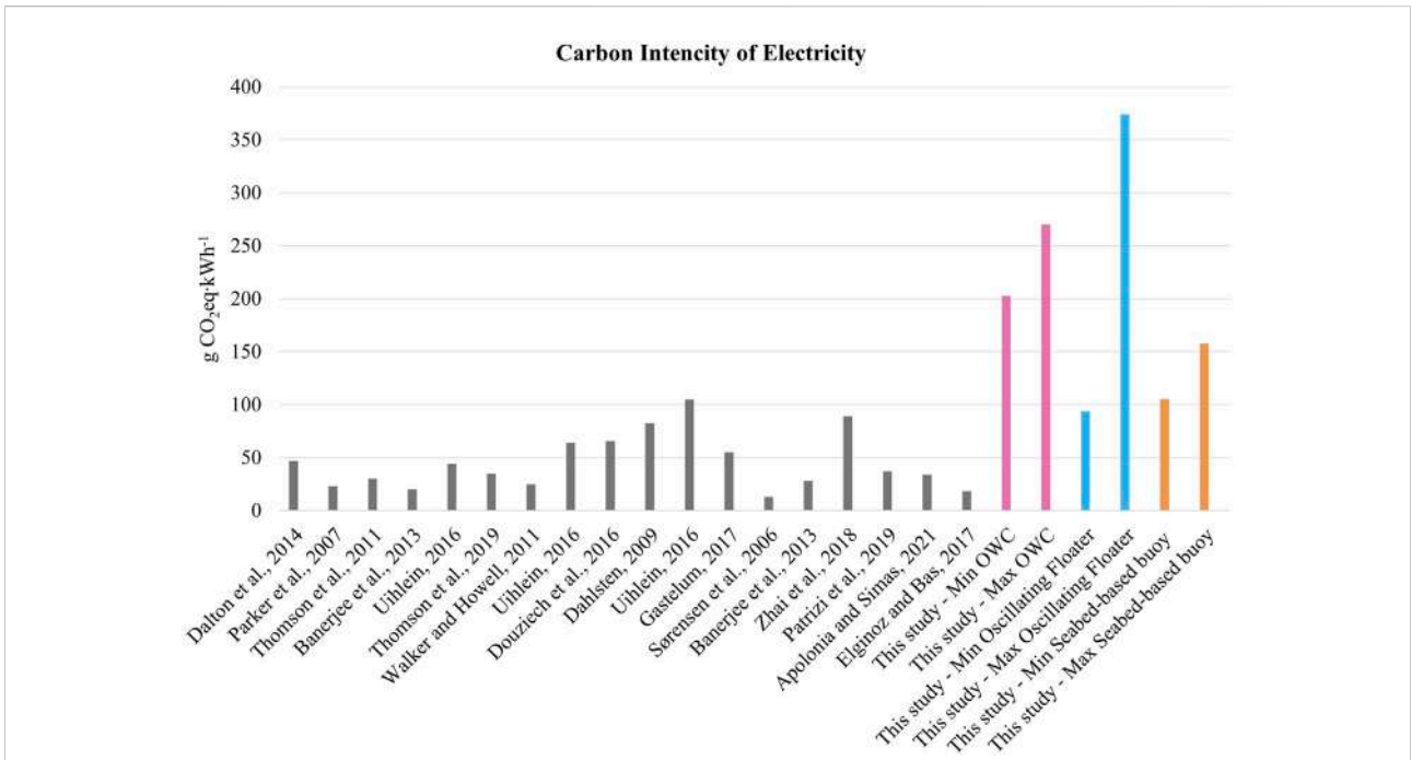
FIGURE 6 CIE values of the WEC systems available in the literature (grey columns) and results obtained from the present study (colored columns).
