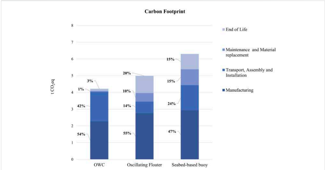
FIGURE 5 Carbon Footprint (t CO 2 eq) results in the three WECs in relation to the different LCA phases analyzed.
