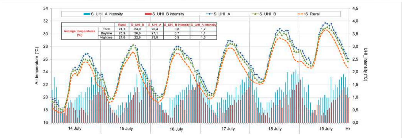
FIGURE 7 | Outdoor temperatures of rural and urban weather in case UHI_1 or UHI_2 on 6 days in July and corresponding UHI intensities. Their average values in the three daily periods are also shown.
