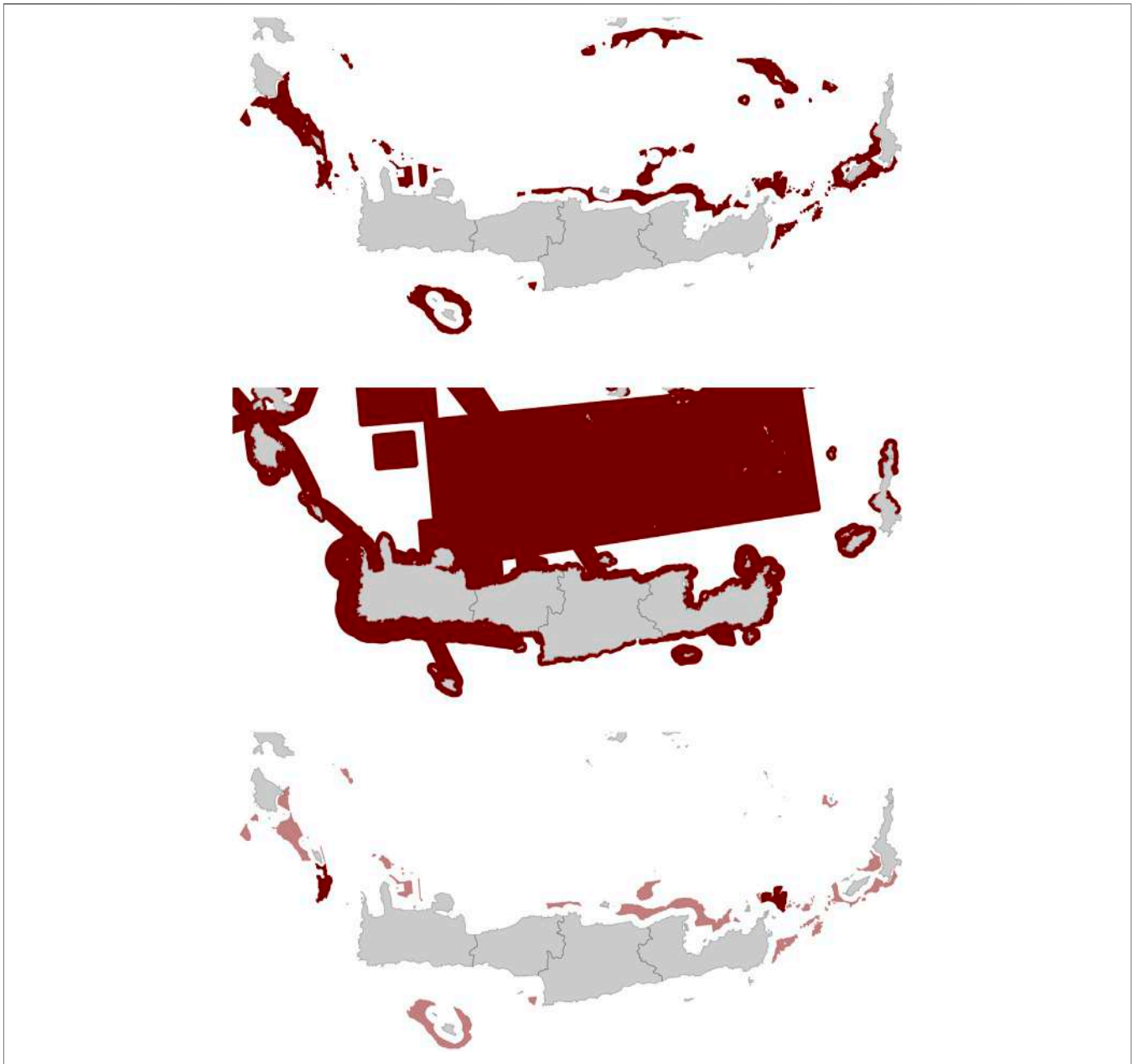
FIGURE 1 | Sequence of maps showing the process for the identification of potential sites for the installation of offshore wind turbines in Crete: a. Combination of bathymetry (50–400 m) and wind speed (>4 m/s); b. Exclusion zones: the union of areas with high ecological value (2 km buffer zone), main navigation routes, and maneuvering areas of ports (5 km buffer zone); c. Eligible areas (in light red) from the combination of the two previous maps and pilot sites (optimal wind speed \geq 7 m/s at 100 m above sea level).
