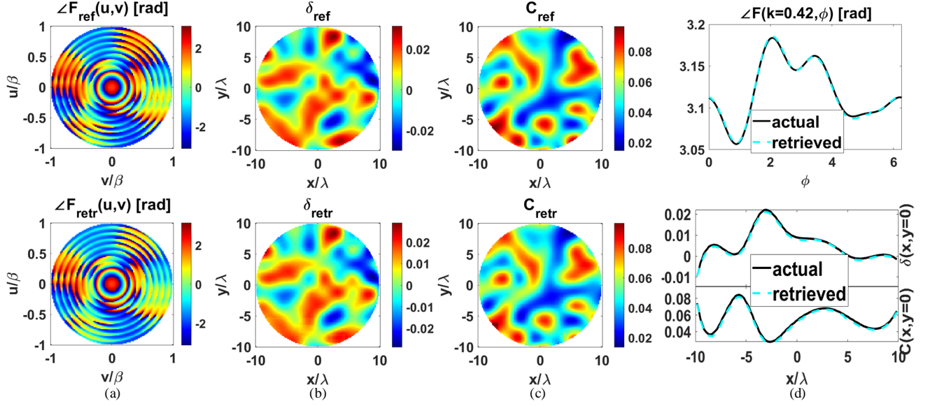
Fig. 4. Assessment scenario #2: amplitude and phase distortion on aperture field ( u = k \cos \phi , v = k \sin \phi ). From left to right: (a) reference (top) and retrieved (bottom) phase of the radiated far-field; (b) reference (top) and retrieved (bottom) reflector surface deformation; (c) reference (top) and retrieved (bottom) amplitude deformation; (d) 1-D cuts of the reference (black curve) and retrieved (dashed-cyan curve) far-field phase along the ring at k = 0.4189 (top) and surface and amplitude deformations along y = 0 (bottom).
