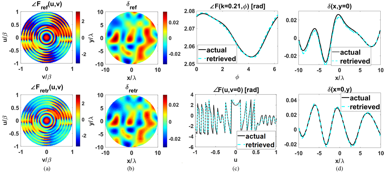
Fig. 3. Assessment scenario #1 in presence of noisy data (SNR=25dB): phase distortion on aperture field ( u = k \cos \phi , v = k \sin \phi ). From left to right: (a) reference (top) and retrieved (bottom) phase of the radiated far-field; (b) reference (top) and retrieved (bottom) reflector surface deformation; (c) 1-D cuts of the reference (black curve) and retrieved (dashed-cyan curve) far-field phase along the ring at k = 0.2094 (top) and the diameter v = 0 (bottom); (d) 1-D cuts of the reference (black curve) and retrieved (dashed-cyan curve) surface deformation along y = 0 (top) and x = 0 (bottom).
