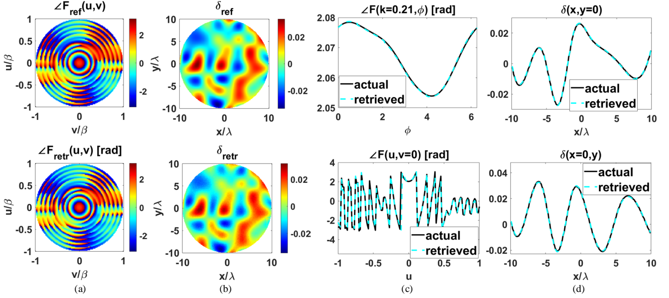
Fig. 2. Assessment scenario #1: phase distortion on aperture field ( u = k \cos \phi , v = k \sin \phi ). From left to right: (a) reference (top) and retrieved (bottom) phase of the radiated far-field; (b) reference (top) and retrieved (bottom) reflector surface deformation; (c) 1-D cuts of the reference (black curve) and retrieved (dashed-cyan curve) far-field phase along the ring at k = 0.2094 (top) and the diameter v = 0 (bottom); (d) 1-D cuts of the reference (black curve) and retrieved (dashed-cyan curve) surface deformation along y = 0 (top) and x = 0 (bottom).
