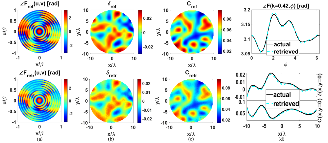
Fig. 5. Assessment scenario #2 in presence of noisy data (SNR=25dB): amplitude and phase distortion on aperture field ( u = k \cos \phi , v = k \sin \phi ). From left to right: (a) reference (top) and retrieved (bottom) phase of the radiated far-field; (b) reference (top) and retrieved (bottom) reflector surface deformation; (c) reference (top) and retrieved (bottom) amplitude deformation; (d) 1-D cuts of the reference (black curve) and retrieved (dashed-cyan curve) far-field phase along the ring at k = 0.4189 (top) and surface and amplitude deformations along y = 0 (bottom).
