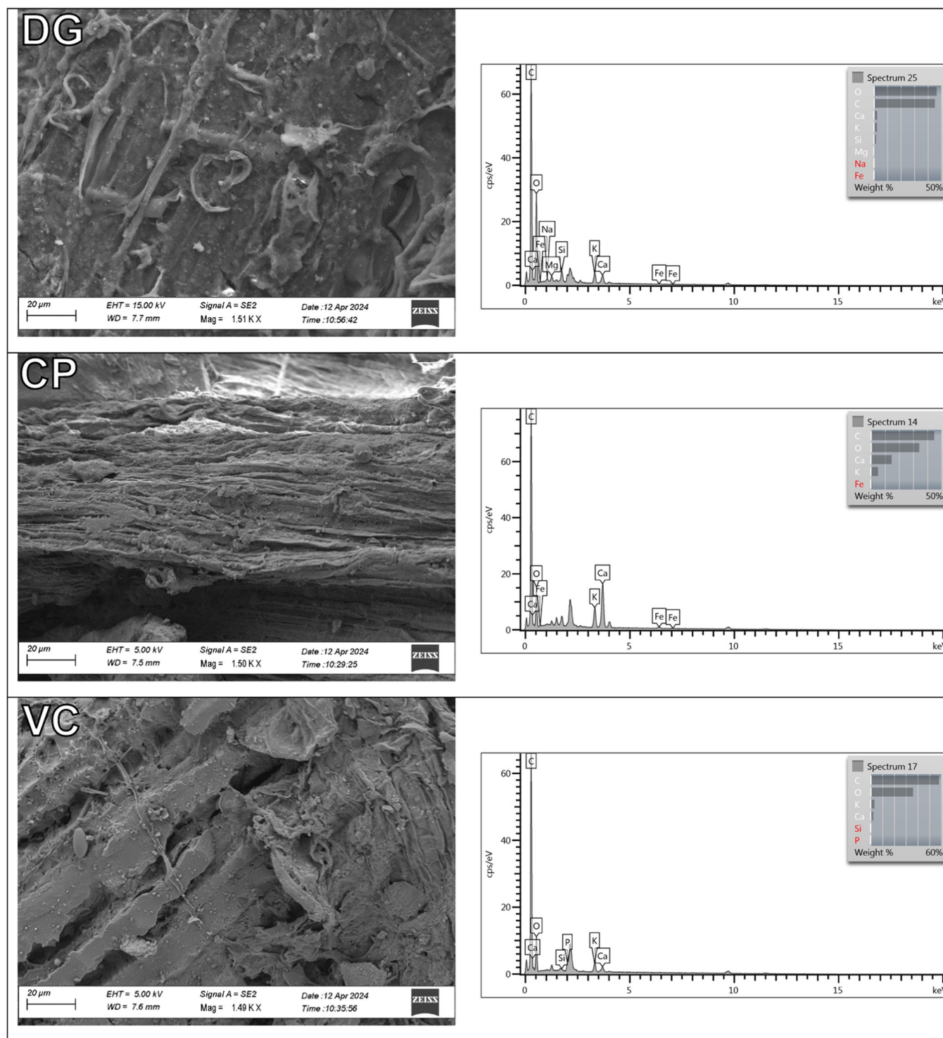
FIGURE 1 Scanning electron micrographs at magnifications of 1500 \times and energy-dispersive X-ray (EDX) spectra of the materials. Images were taken with secondary electrons. CP, compost; DG, solid digestate; VC, vermicompost.
