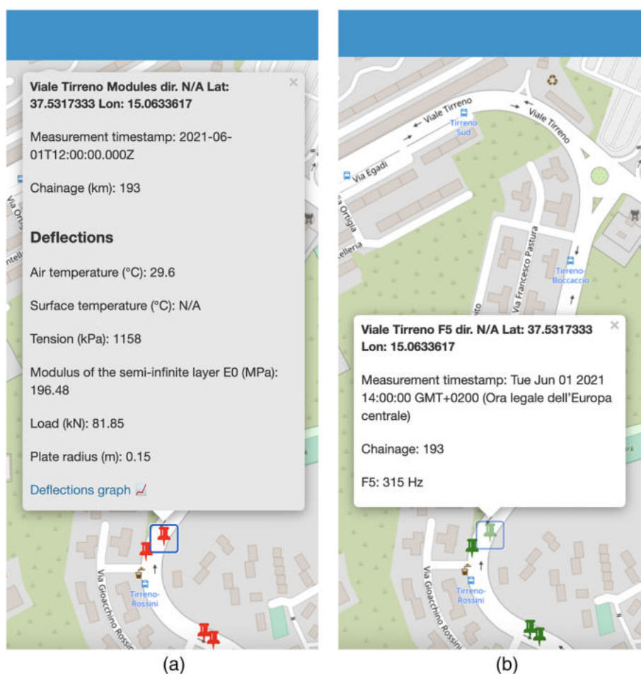
FIGURE 10 Condition data shown in the web-platform: (a) asphalt layer moduli; (b) NDT-SHM f5 values.
