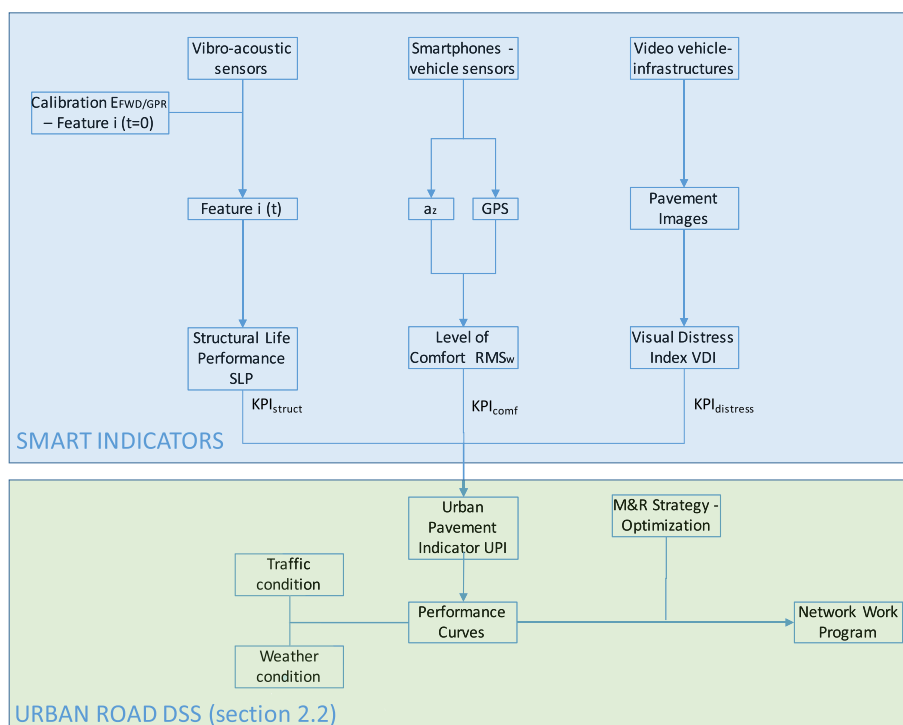
FIGURE 5 Smart indicators and Urban Road Decision Support System. Logic SCHEME
