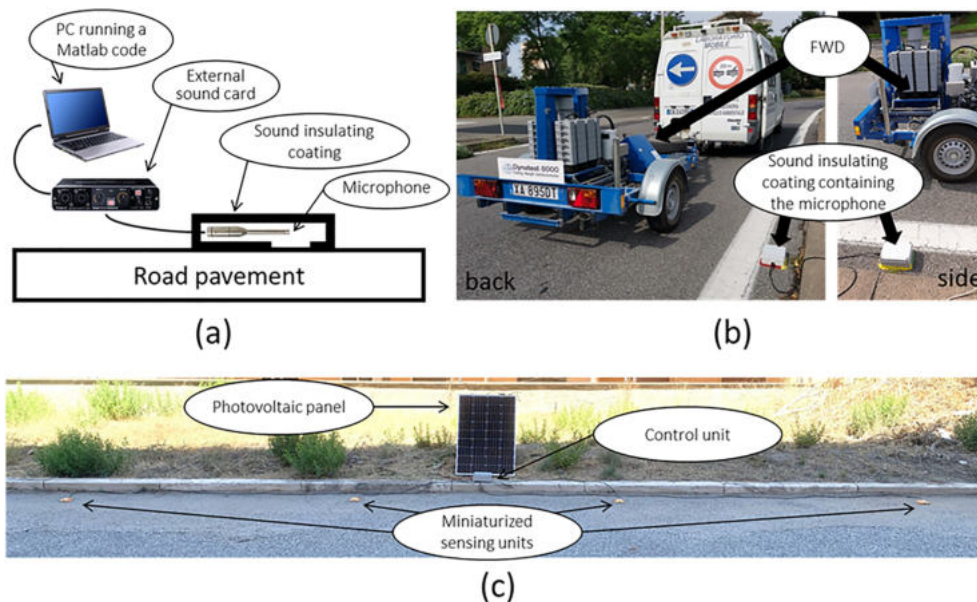
FIGURE 2 Innovative NDT-SHM system (PRIN project USR342). (a) Scheme of the first prototype of the system. (b) First prototype of the system (back and side view) during the tests carried out in Catania (Task 2 of the PRIN project USR342). (c) The Second prototype of the NDT-SHM system during its setup
