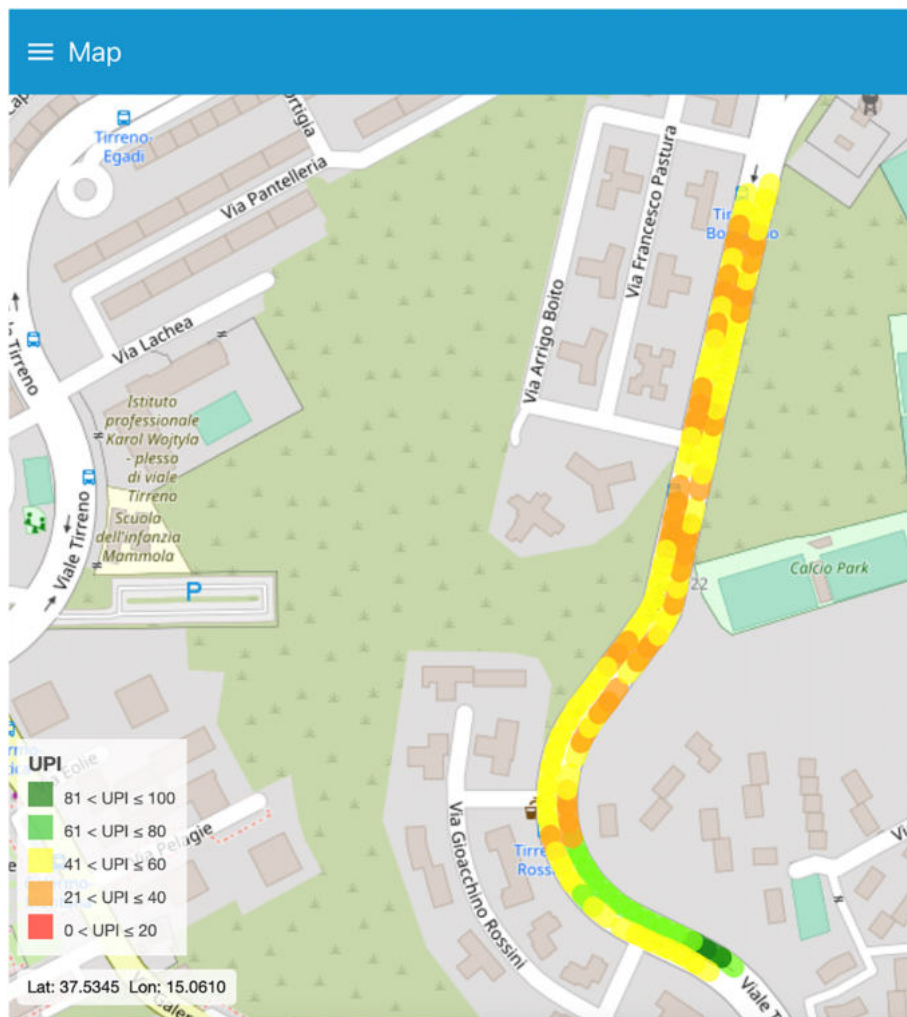
FIGURE 13 UPI along the selected road segment
