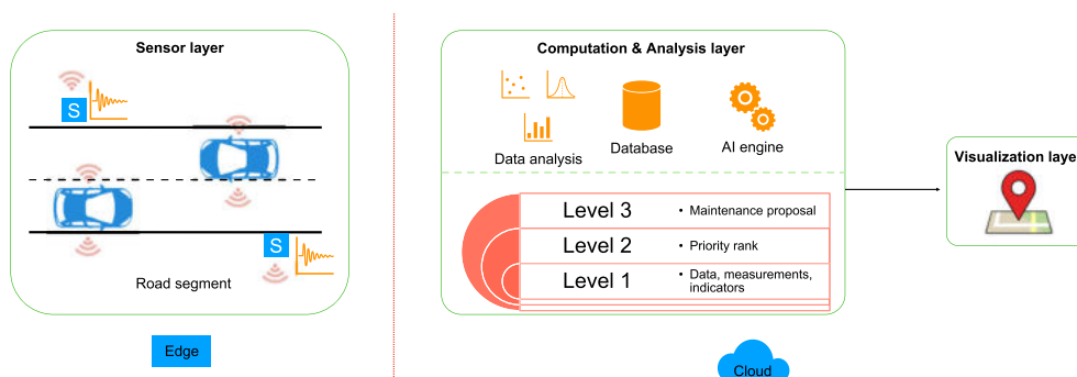
FIGURE 6 Platform architecture
