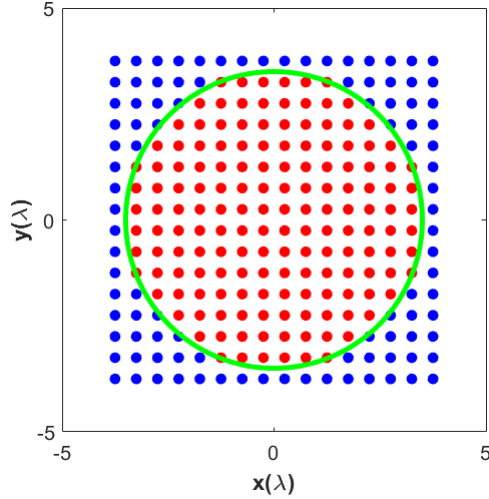
Fig. 3.3: Array layout (comparison with [7]), where only the elements internal to the circle of radius 3.5\lambda (i.e., depicted in red color) are used.
