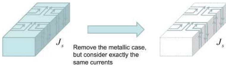
Fig. 1.3: Non radiating sources: an example.
