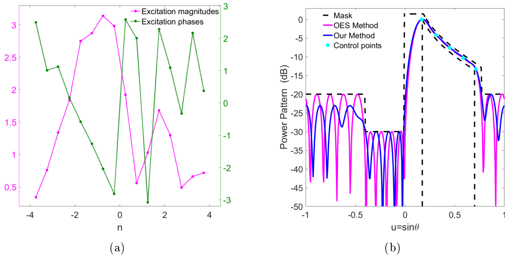
Fig. 2.3: Comparison with [3]: excitations set synthesized through the proposed method (a) and comparison between the power pattern corresponding to them and the OES solution (b).
