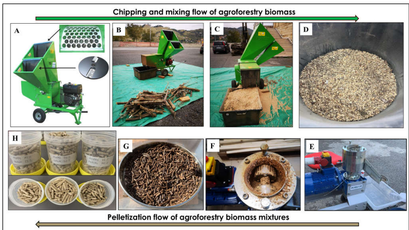
Figure 1. Flow of the chipping and pelletizing processes of agroforestry pruning residues: (A) Chipper/Shredder “Peruzzo model T3; (B) start of the chipping phase of olive tree pruning residues; (C) completion of the chipping phase of olive tree pruning residues; (D) mixing process of different agroforestry wood residues; (E) rotating roller pelletizer (Peruzzo model Minipel E80); (F) detail of the rollers of the pelleting machine during the pelletizing phase; (G) freshly produced olive wood pellets (100%) in the cooling phase; and (H) samples of pellets made with different percentage blends of poplar and citrus.
