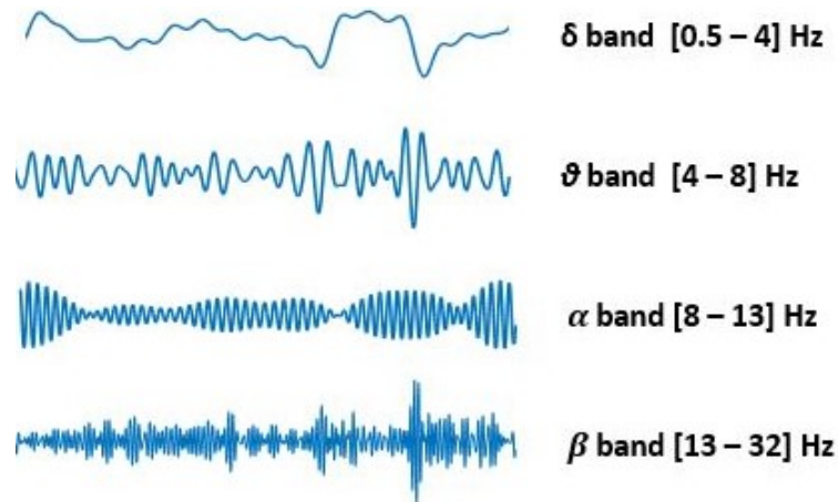
Fig. 1.3: EEG sub-bands.
