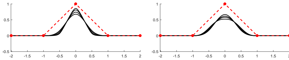
Figure 4: From lower to taller functions: basic limit functions for the space EP_T = \text{span}\{1, t, e^{\theta t}, e^{-\theta t}\} with \theta \in \{i, 3i, 5i, 7i\} (left), \theta \in \{3, 2.5, 2, 0\} (right), obtained from the initial data set represented by a dashed line.
