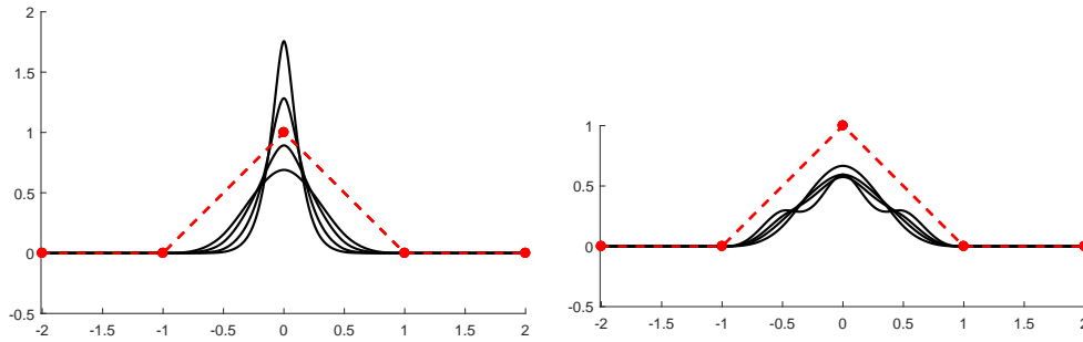
Figure 5: From lower to taller functions: basic limit functions for the space EP_T = \text{span}\{e^{\theta t}, e^{-\theta t}, te^{\theta t}, te^{-\theta t}\} with \theta \in \{i, 3i, 5i, 7i\} (left), \theta \in \{3, 2.5, 2, 0\} (right), obtained from the initial data set represented by a dashed line.
