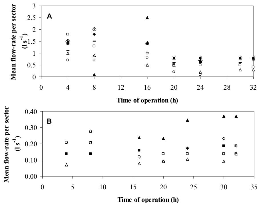
Fig. 3 Mean flow-rate per sector during Trial 2 (A), ◇ T2-S75, □ T2-S120, △ T2-S150, ○ T2-S180, * T2-D40, ◆ T2-D80, ▲ T2-D120,–T2-D140, and Trial 3 (B), ◆ T3-D40, ■ T3-D80, ▲ T3-D120, ◇ T3-S50, △ T3-S120.
