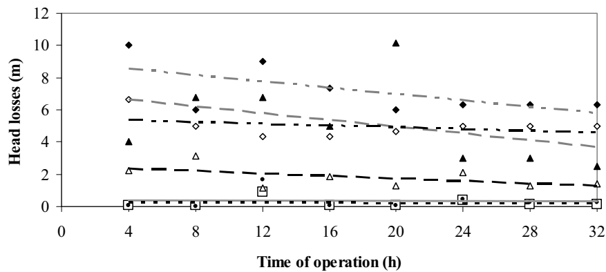
Fig. 2 Head losses in the different trials (T) and filter types (D= disk; S= screen). □ Mean T1-D, * Mean T1-S, △ Mean T2-D, ▲ Mean T2-S, ◇ Mean T3-D, ◆ Mean T3-S.
