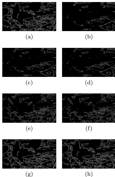
Fig. 10: IR image: ED performed by (a) the proposed approach; (b), (c), and (d) by the Roberts, Prewitt, and Sobel approaches; (e), (f), (g) and (h) by the LoG, Zero-Cross, Canny and Canny & Otsu procedures.
