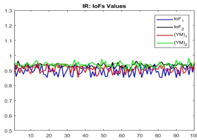
Fig. 6: IoF for IR images.
