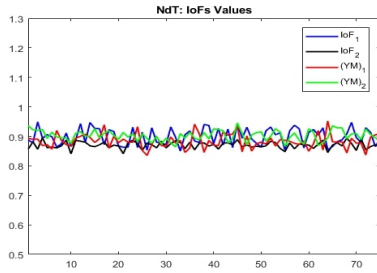
Fig. 5: IoF for EC maps.
