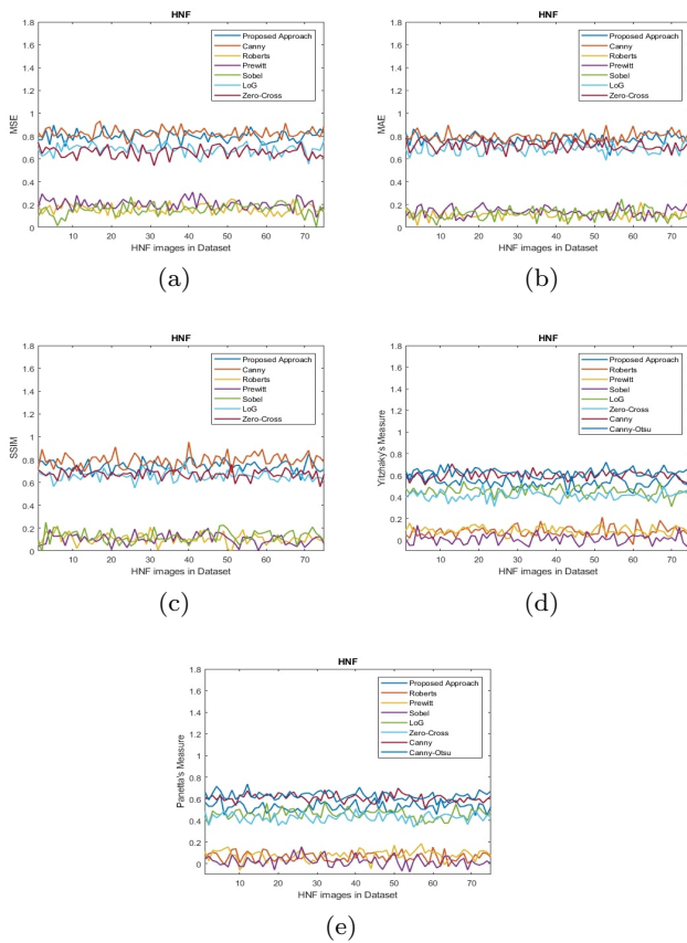
Fig. 13: QAMs for HNF images: (a) MSE, (b) MAE, (c) SSIM, (d) Yitzhaky's measure, (e) Panetta's measure.
