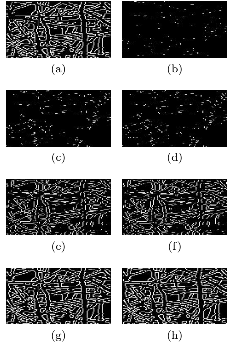
Fig. 12: HNF SEM image: ED performed by (a) the proposed approach; (b), (c), and (d) by the Roberts, Prewitt, and Sobel approaches; (e), (f), (g) and (h) by the LoG, Zero-Cross, Canny and Canny & Otsu procedures.
