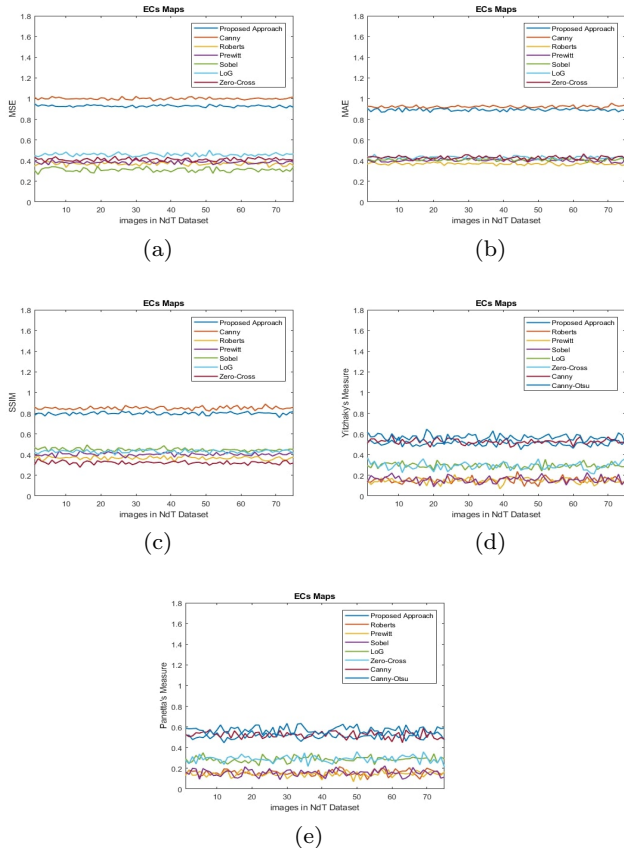
Fig. 9: QAMs for EC maps: (a) MSE, (b) MAE, (c) SSIM, (d) Yitzhaky's measure, (e) Panetta's measure.
