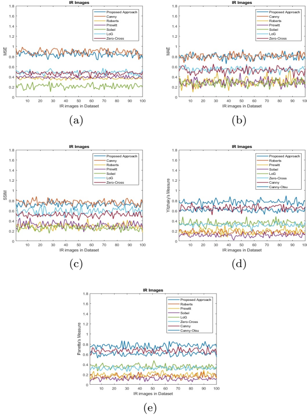
Fig. 11: QAMs for IR images: (a) MSE, (b) MAE, (c) SSIM, (d) Yitzhaky's measure, (e) Panetta's measure.
