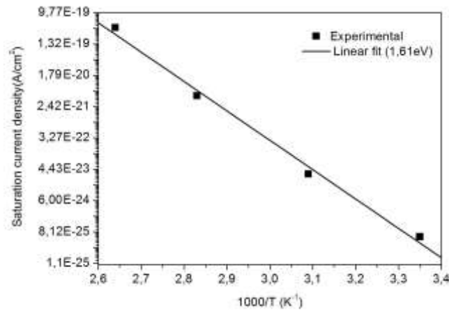
Figure 5. Arrhenius plot of the diode D1A saturation current density.
