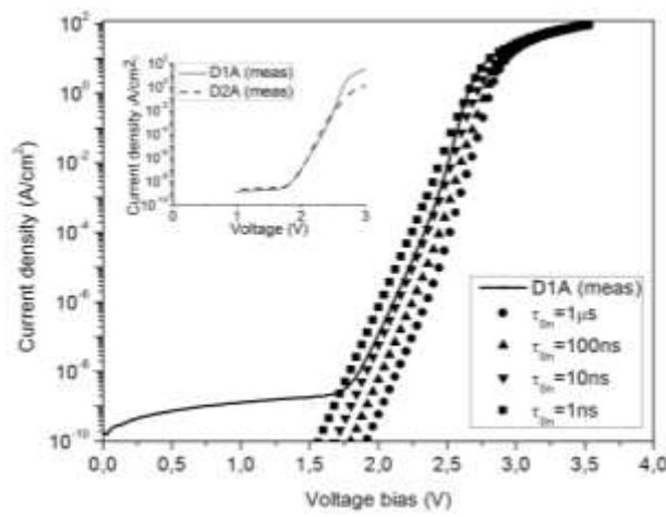
Figure 3. Calibration of the carrier lifetime simulation parameters for the diode D1A at T=298\text{K} . The inset shows a comparison between the measured J - V curves of the diodes D1A and D2A.
