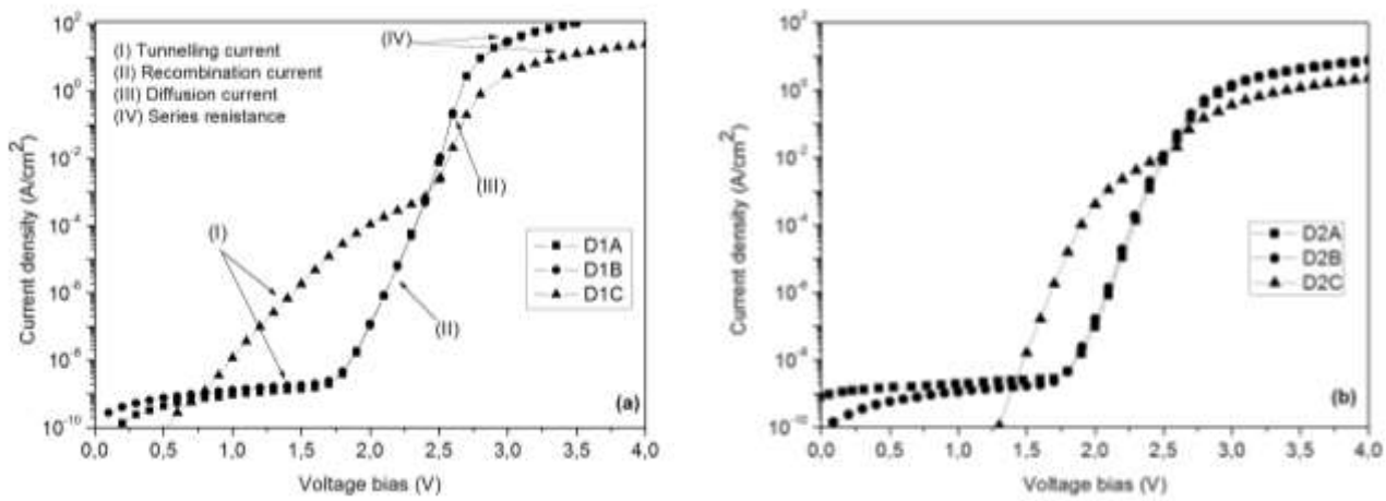
Figure 2. Forward J - V characteristics of several 4H-SiC p-i-n diodes (structure #1 (a), structure #2 (b)) measured at 298K.
