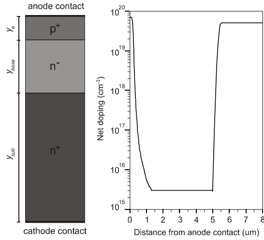
Figure 1. 4H-SiC p-i-n diode schematic cross-section and net doping profile of a device with a 3 \times 10^{15} \text{ cm}^{-3} -doped epilayer.
