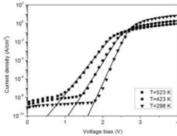
Figure 7. Simulated (solid lines) and experimental (dotted lines) forward characteristics of the diode D2A at different temperatures.
