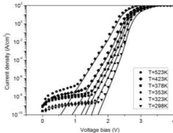
Figure 4. Simulated (solid lines) and experimental (dot lines) forward characteristics of the diode D1A at different temperatures.
