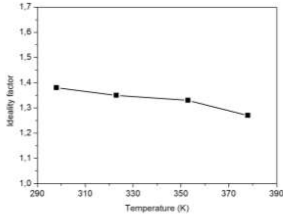
Figure 6. Ideality factor of the diode D1A between 2.5V and 2.75V at different temperatures.
