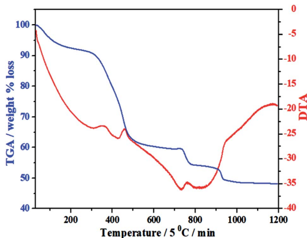
Fig. 1 TG/DTA of mixed-milled nitrates xerogel.
