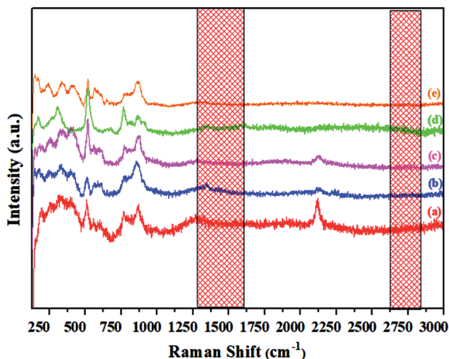
Fig. 11 Raman spectra of the molten C_{12}A_7-xV_x:e^- where x = (a) 0.25 V, (b) 0.50 V, (c) 0.75 V, (d) 1 V, (e) 1.5 V.
