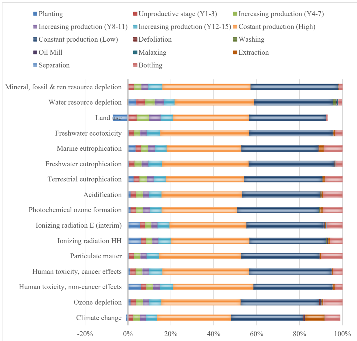
Fig. 8. Dominance analysis for the HC scenario
