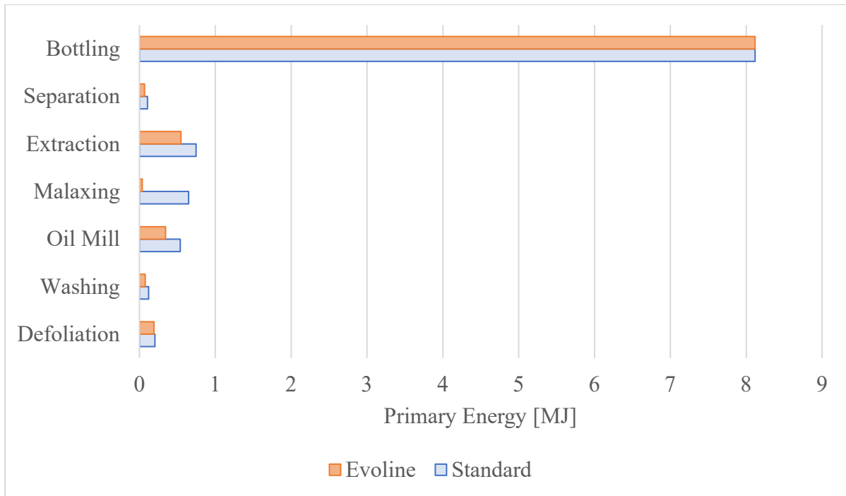
Fig. 7. Dominance analysis on life cycle energy for the transformation stage between the “Evoline” and standard approach
