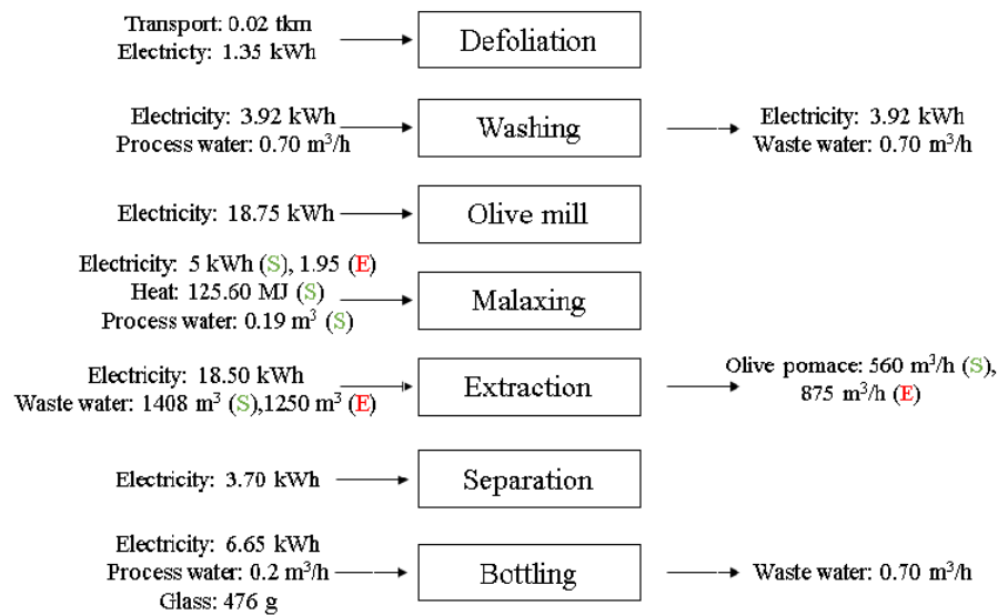
Fig. 3. Modelling assumptions in the transformation stages
